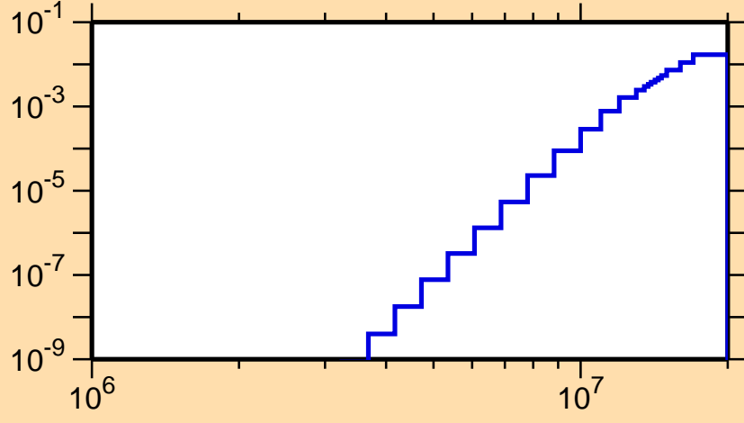
\sigma vs. E for ^{180}\text{Ir}(n,n\alpha)
