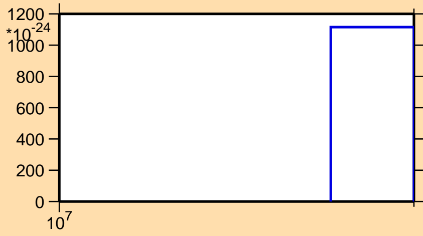
\sigma vs. E for ^{180}\text{Ir} (mt 42)
