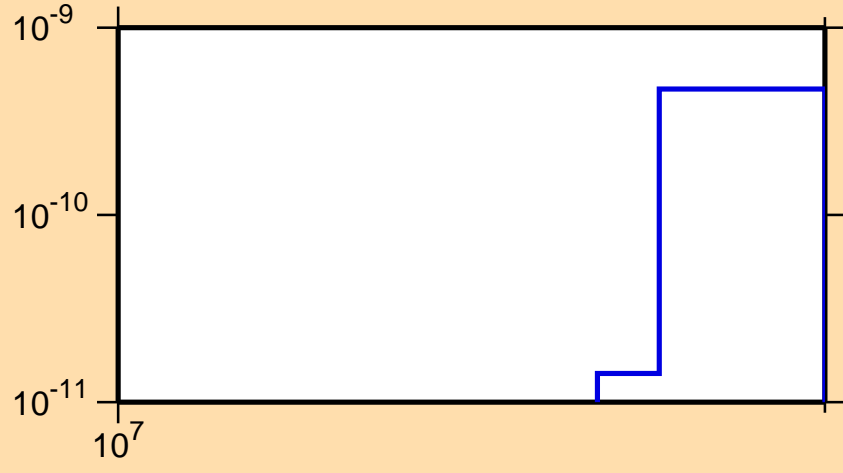
\sigma vs. E for ^{180}\text{Ir} (mt 34)
