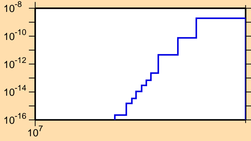
\sigma vs. E for ^{180}\text{Ir}(n,\text{pt})
