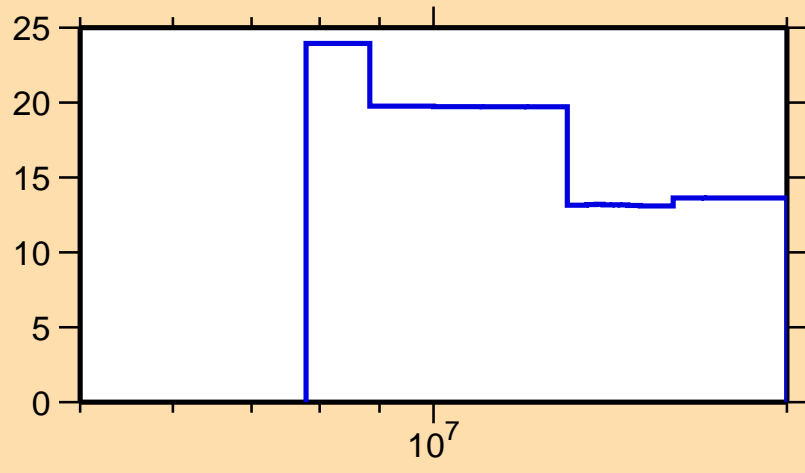
\Delta\sigma/\sigma vs. E for ^{180}\text{Ir}(n,2n)
