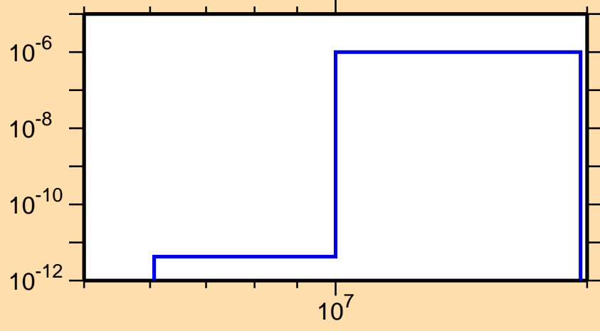
\sigma vs. E for ^{180}\text{Ir}(n,\text{He}3)
