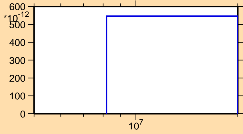
\sigma vs. E for ^{180}\text{Ir}(\text{mt117})
