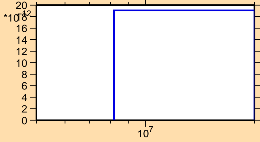
\sigma vs. E for ^{180}\text{Ir}(n,\text{pt})
