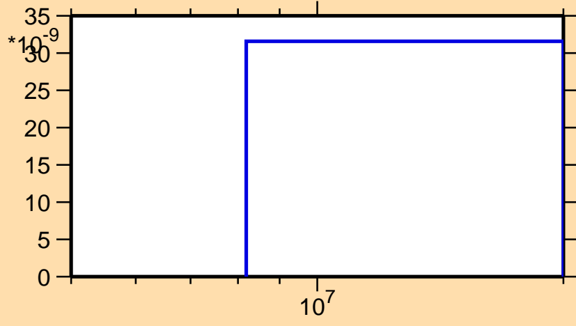
\sigma vs. E for ^{180}\text{Ir}(\text{mt } 45)
