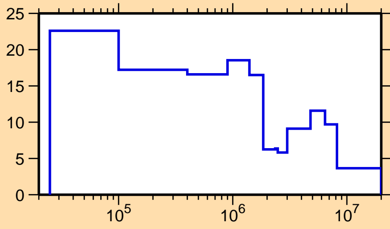
\Delta\sigma/\sigma vs. E for ^{180}\text{Ir}(n,\text{tot.})
