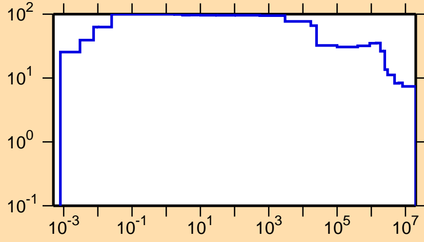
\Delta\sigma/\sigma vs. E for ^{180}\text{Ir}(n,\text{nonel.})
