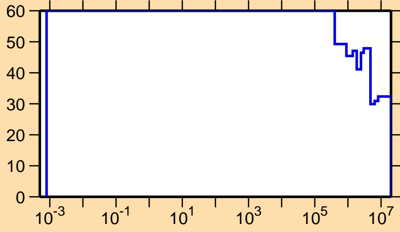
\Delta\sigma/\sigma vs. E for ^{180}\text{Ir}(n,p)
