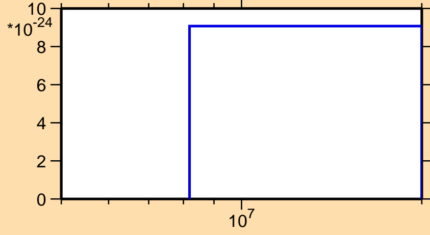
\sigma vs. E for ^{180}\text{Ir}(\text{mt } 42)
