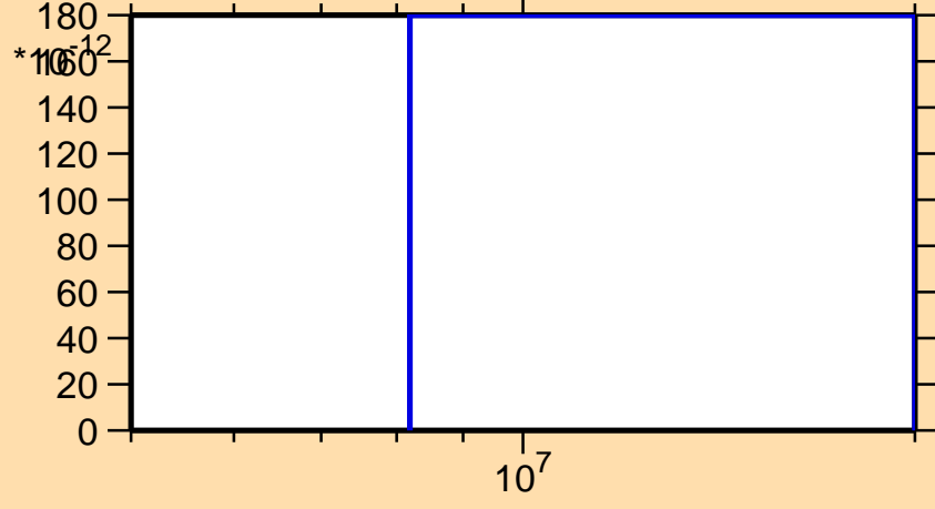
\sigma vs. E for ^{180}\text{Ir}(n,\text{pd})
