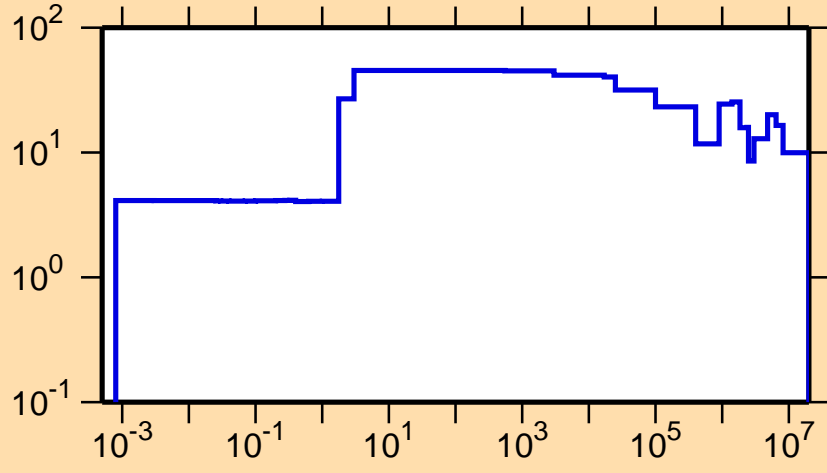
\Delta\sigma/\sigma vs. E for ^{180}\text{Ir}(n,el.)
