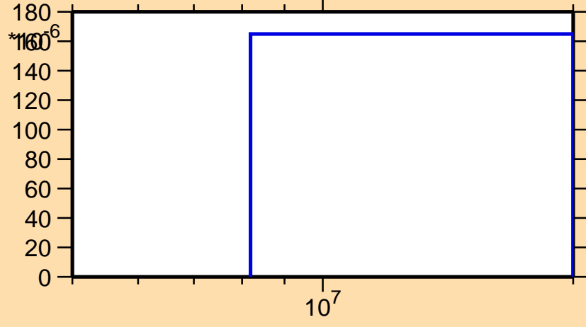
\sigma vs. E for ^{180}\text{Ir}(n,2np)
