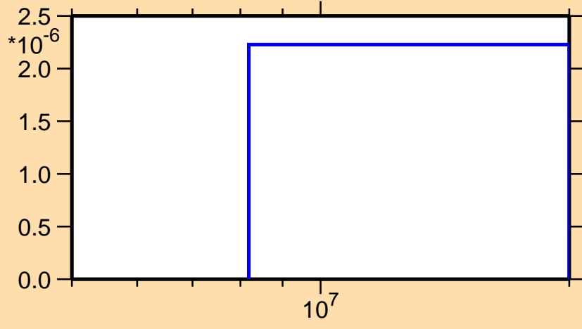
\sigma vs. E for ^{180}\text{Ir}(n,3n)
