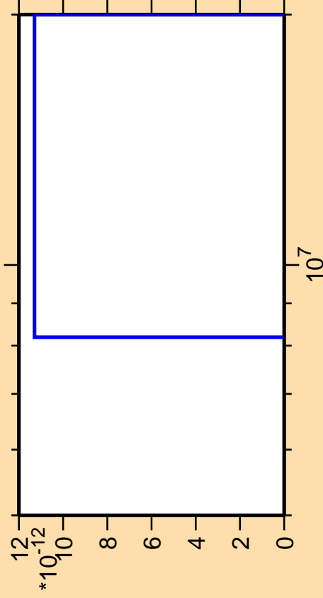
\Delta\sigma/\sigma vs. E for ^{180}\text{Ir}(\text{mt } 42)
