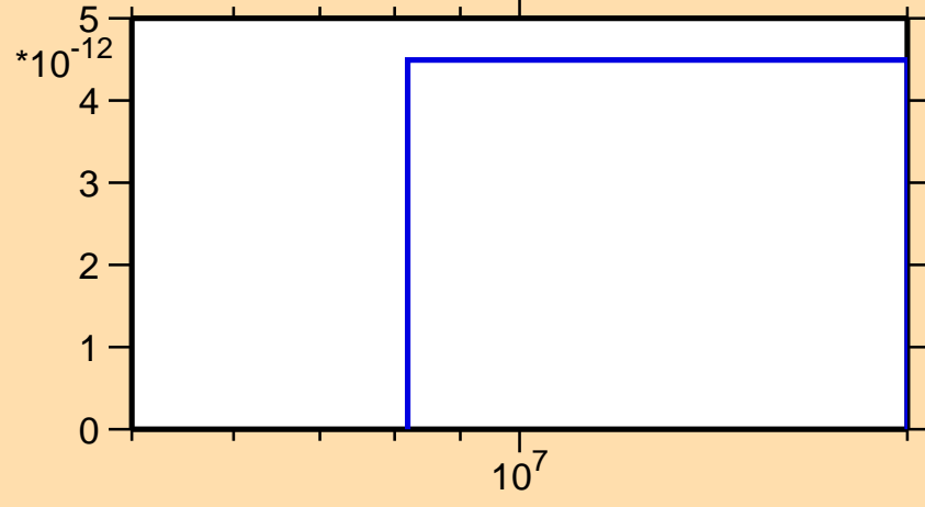
\sigma vs. E for ^{180}\text{Ir}(\text{mt } 34)
