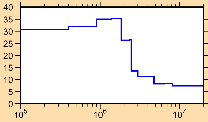
\Delta\sigma/\sigma vs. E for ^{180}\text{Ir}(n,\text{nonel.})
