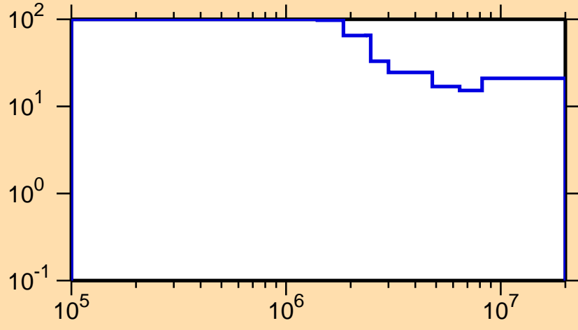
\Delta\sigma/\sigma vs. E for ^{180}\text{Ir}(n,n\text{cont.})
