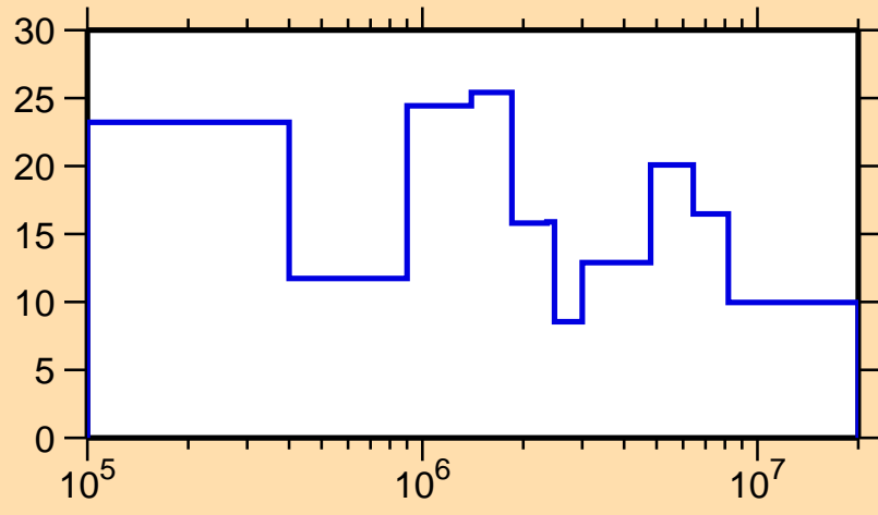
\Delta\sigma/\sigma vs. E for ^{180}\text{Ir}(n,\text{el.})
