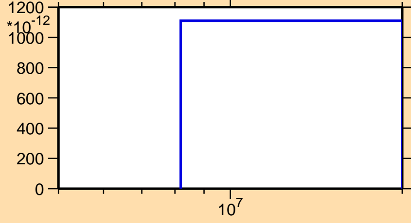
\sigma vs. E for ^{180}\text{Ir}(n,nt)
