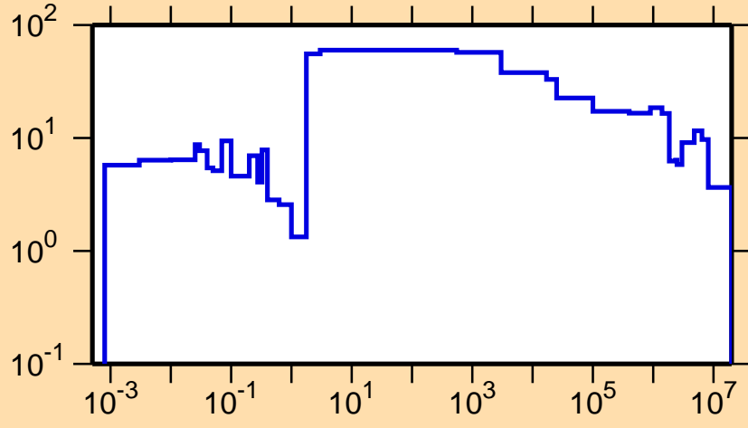
\Delta\sigma/\sigma vs. E for ^{180}\text{Ir}(n,\text{tot.})
