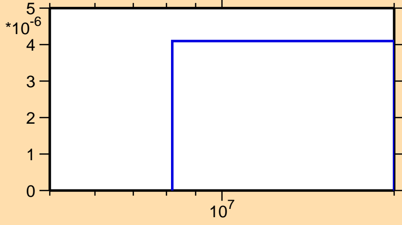
\sigma vs. E for ^{180}\text{Ir}(n,2n\alpha)
