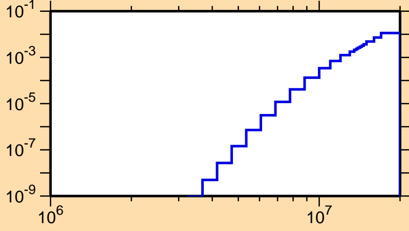
\sigma vs. E for ^{181}\text{Ir}(n,n\alpha)
