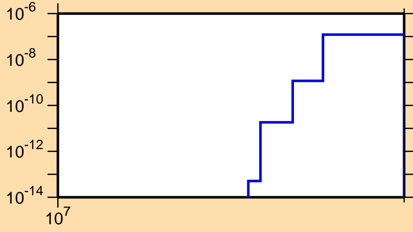
\sigma vs. E for ^{181}\text{Ir}(n,nt)
