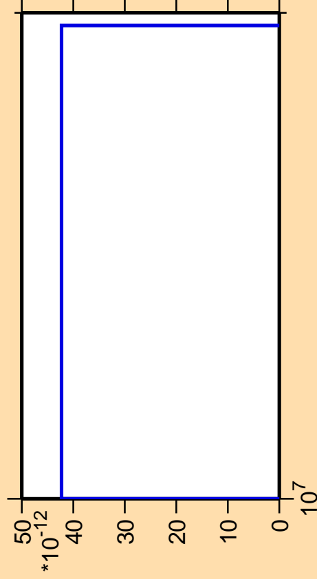
\Delta\sigma/\sigma vs. E for ^{181}\text{Ir} (mt 42)
