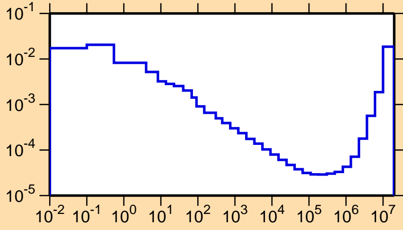
\sigma vs. E for ^{181}\text{Ir}(n,\alpha)
