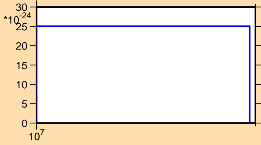
\sigma vs. E for ^{181}\text{Ir} (mt 42)
