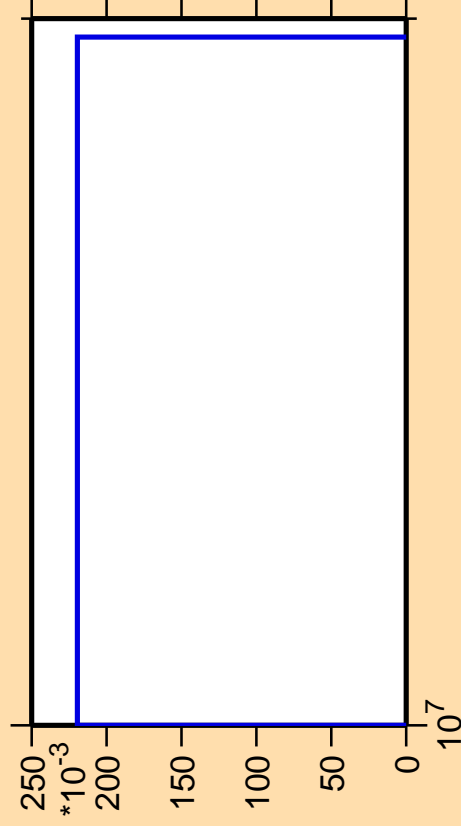
\Delta\sigma/\sigma vs. E for ^{181}\text{Ir} (mt 34)
