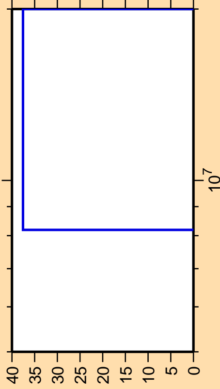
\Delta\sigma/\sigma vs. E for ^{181}\text{Ir}(n,p)
