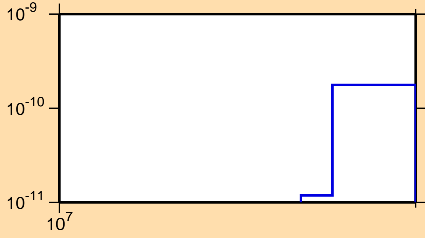
\sigma vs. E for ^{183}\text{Ir}(n,\text{pd})
