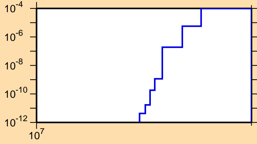
\sigma vs. E for ^{183}\text{Ir}(n,2np)
