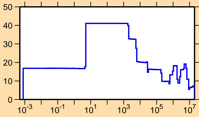
\Delta\sigma/\sigma vs. E for ^{183}\text{Ir}(n,el.)
