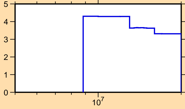
\Delta\sigma/\sigma vs. E for ^{183}\text{Ir}(n,\text{nonel.})
