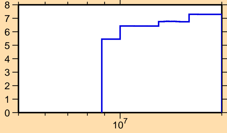
\Delta\sigma/\sigma vs. E for ^{183}\text{Ir}(n,\text{el.})
