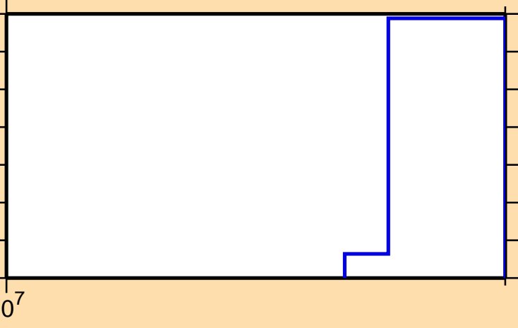
\sigma vs. E for ^{183}\text{Ir}(n,3n)
