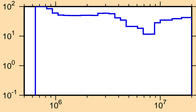
\Delta\sigma/\sigma vs. E for ^{183}\text{Ir}(n,n\text{cont.})
