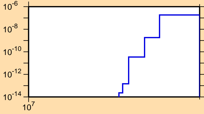
\sigma vs. E for ^{183}\text{Ir}(n,nt)
