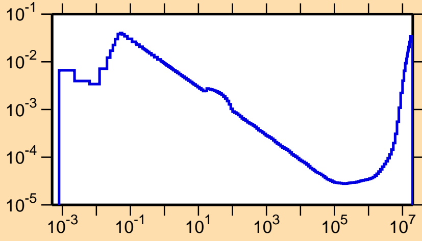
\sigma vs. E for ^{184}\text{Ir}(n,\alpha)
