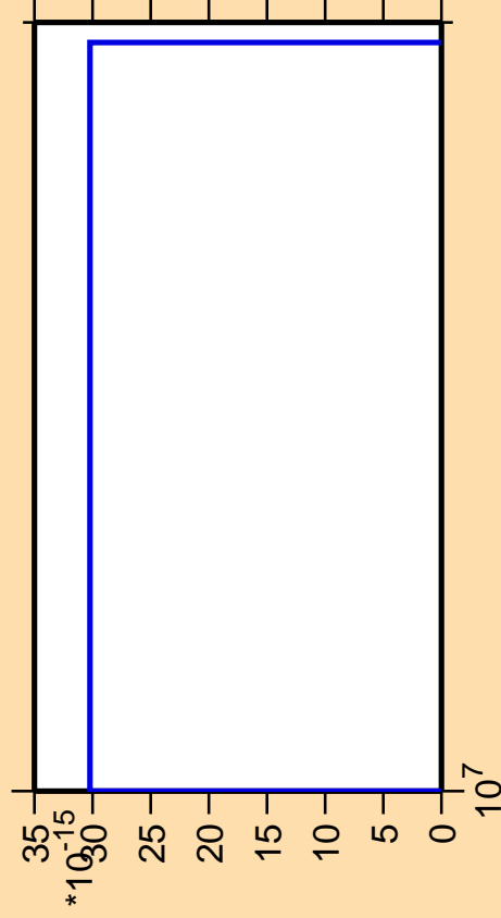
\Delta\sigma/\sigma vs. E for ^{184}\text{Ir} (mt 42)
