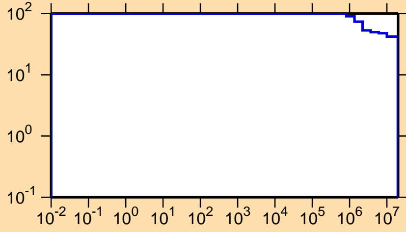
\Delta\sigma/\sigma vs. E for ^{184}\text{Ir}(n,p)
