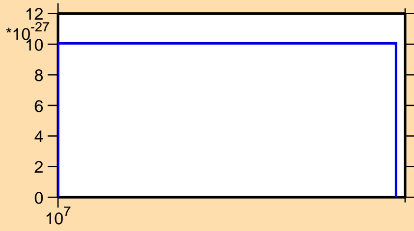
\sigma vs. E for ^{184}\text{Ir} (mt 42)
