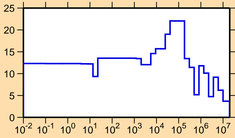
\Delta\sigma/\sigma vs. E for ^{184}\text{Ir}(n,el.)
