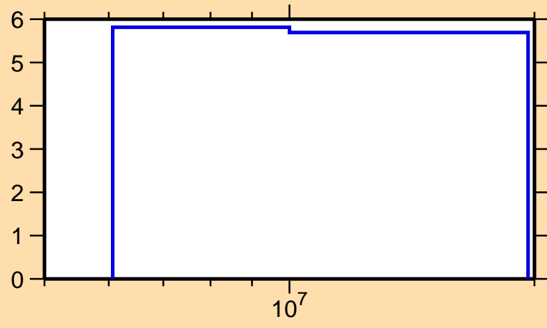
\Delta\sigma/\sigma vs. E for ^{184}\text{Ir}(n,\text{nonel.})
