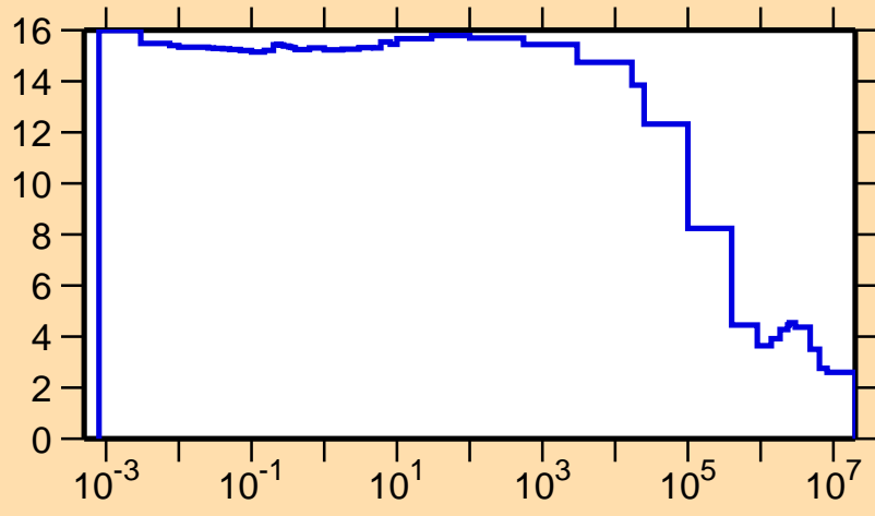
\sigma vs. E for ^{184}\text{Ir}(n,\text{el.})
