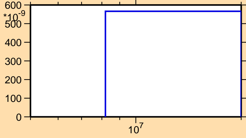
\sigma vs. E for ^{184}\text{Ir}(n,\text{nd})
