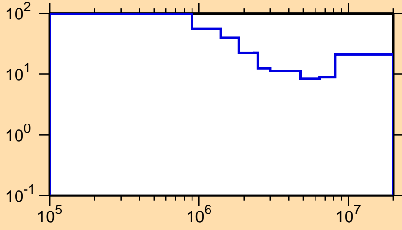
\Delta\sigma/\sigma vs. E for ^{184}\text{Ir}(n,n\text{cont.})
