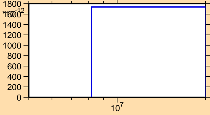
\sigma vs. E for ^{184}\text{Ir}(n,nt)
