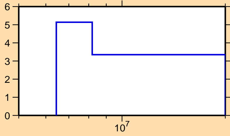
\Delta\sigma/\sigma vs. E for ^{184}\text{Ir}(n,\text{tot.})
