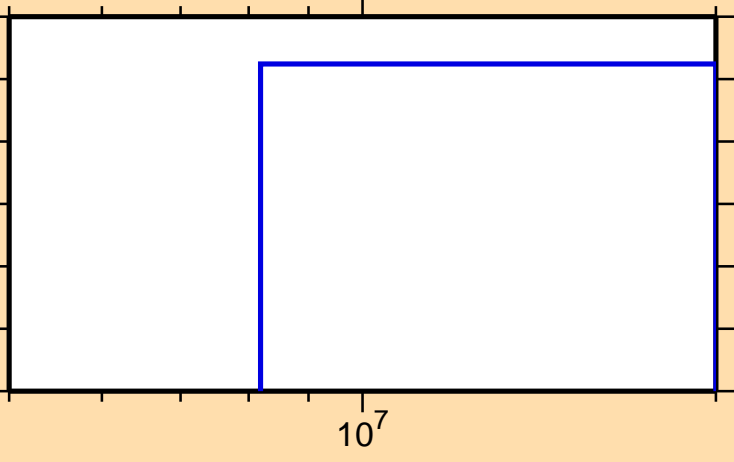
\sigma vs. E for ^{184}\text{Ir}(n,\text{He}3)
