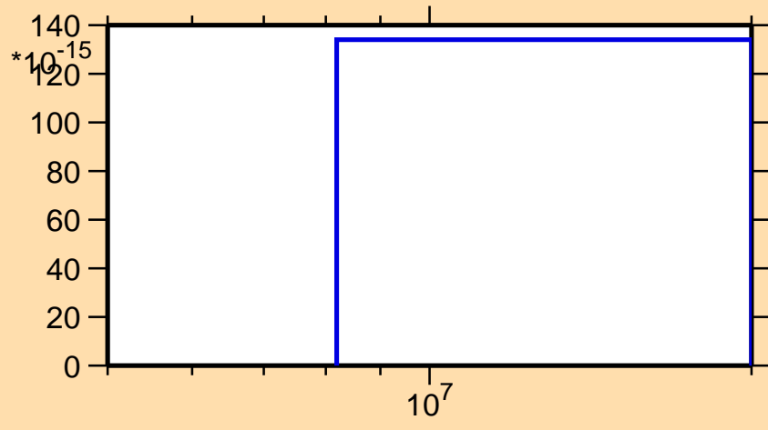
\sigma vs. E for ^{184}\text{Ir}(\text{mt } 34)
