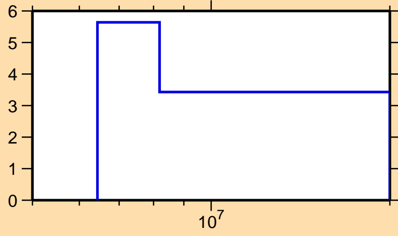
\Delta\sigma/\sigma vs. E for ^{184}\text{Ir}(n,\text{el.})
