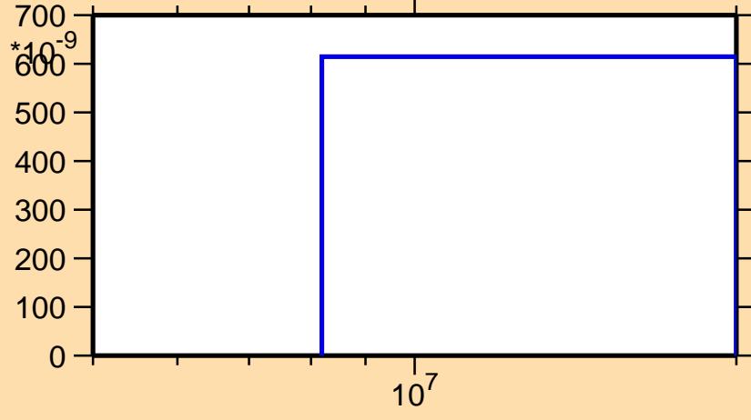
\sigma vs. E for ^{184}\text{Ir}(n,2n\alpha)
