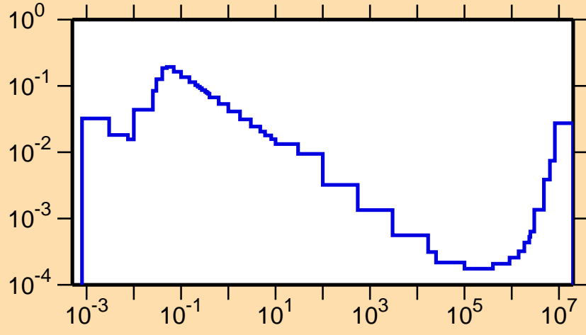
\sigma vs. E for ^{184}\text{Ir}(n,p)
