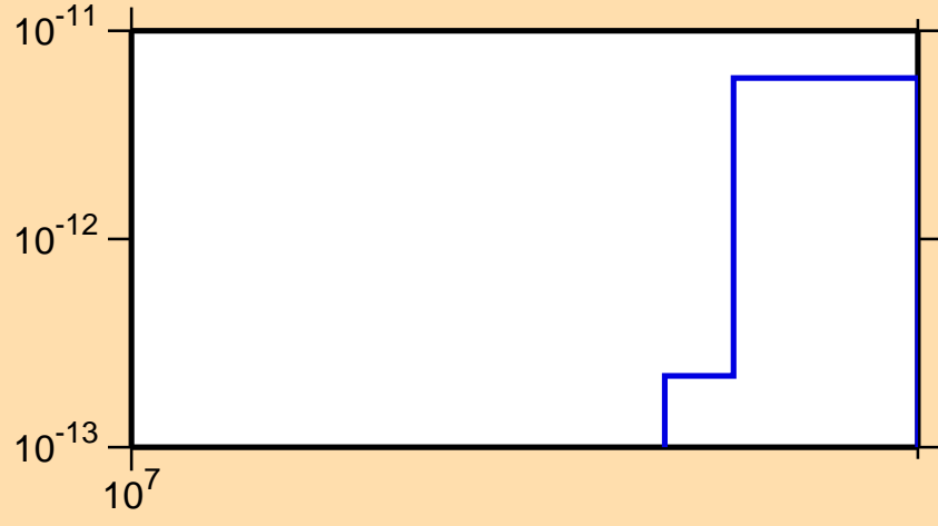
\sigma vs. E for ^{185}\text{Ir}(n,\text{pd})
