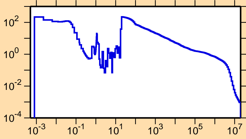
\sigma vs. E for ^{185}\text{Ir}(n,\gamma)
