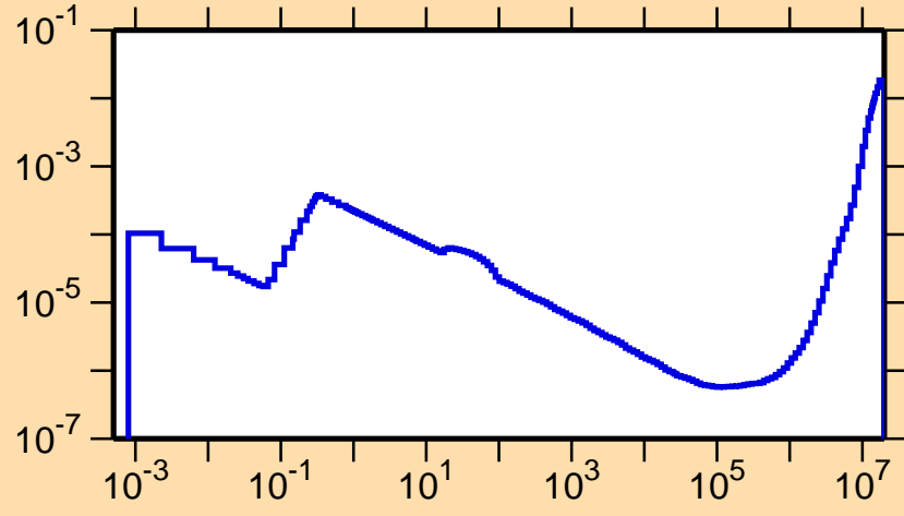
\sigma vs. E for ^{185}\text{Ir}(n,\alpha)
