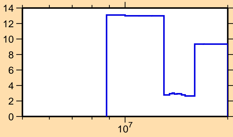
\Delta\sigma/\sigma vs. E for ^{185}\text{Ir}(n,2n)
