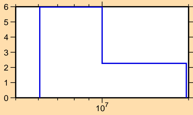
\Delta\sigma/\sigma vs. E for ^{185}\text{Ir}(n,\text{tot.})
