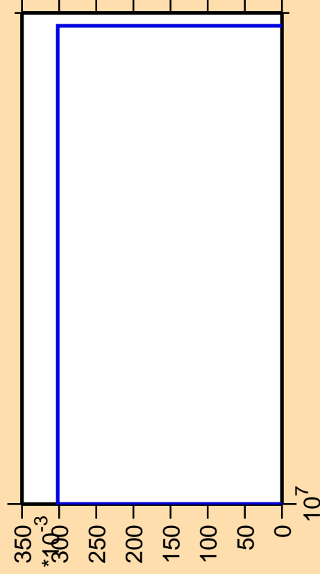
\Delta\sigma/\sigma vs. E for ^{185}\text{Ir}(n,pd)
