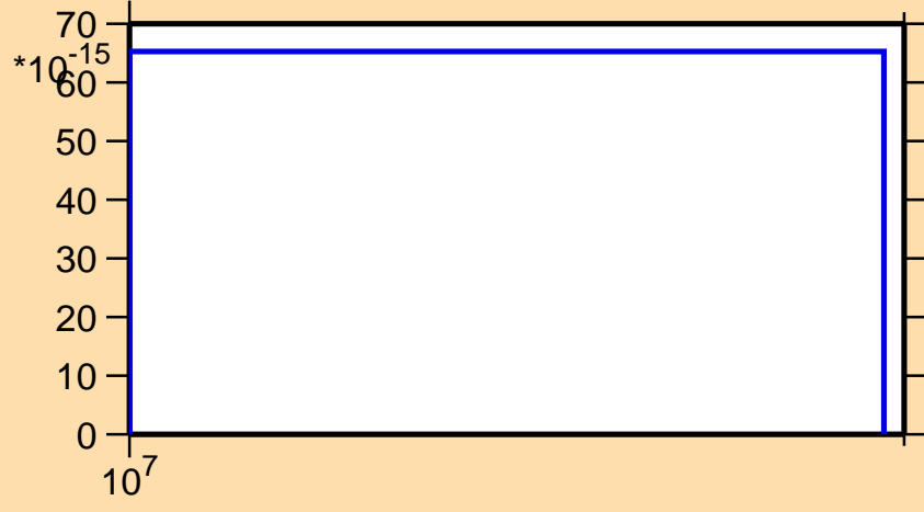
\sigma vs. E for ^{185}\text{Ir}(n,pd)
