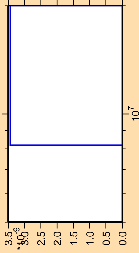
\Delta\sigma/\sigma vs. E for ^{185}\text{Ir}(\text{mt } 42)
