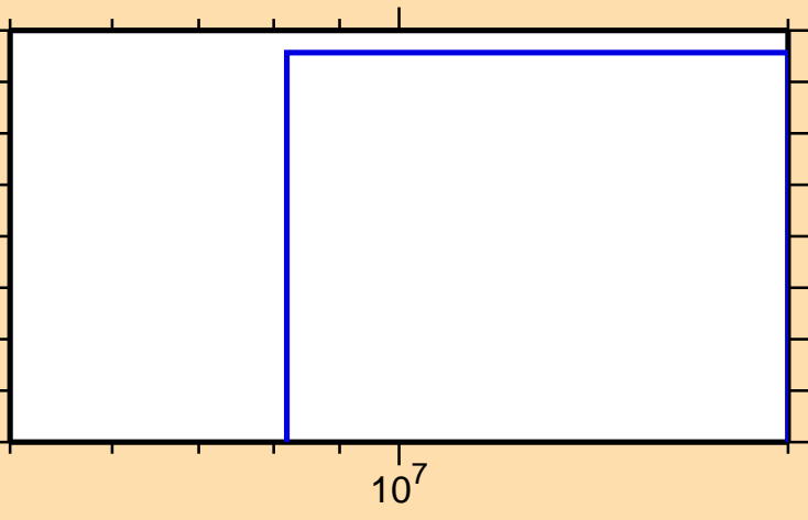
\sigma vs. E for ^{185}\text{Ir}(n,2n\alpha)
