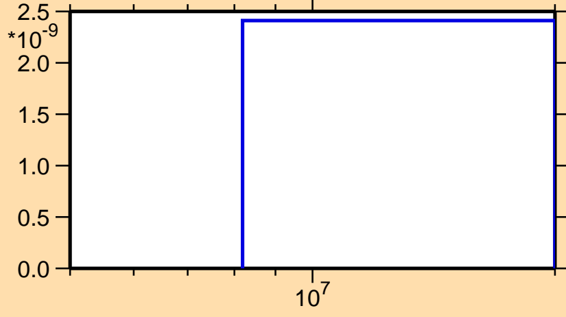
\sigma vs. E for ^{185}\text{Ir}(n,nt)
