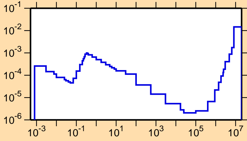
\sigma vs. E for ^{185}\text{Ir}(n,p)
