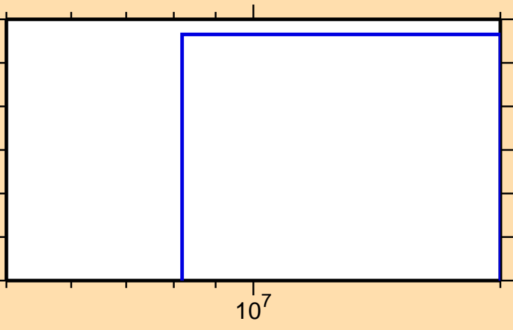
\sigma vs. E for ^{185}\text{Ir}(\text{mt } 34)
