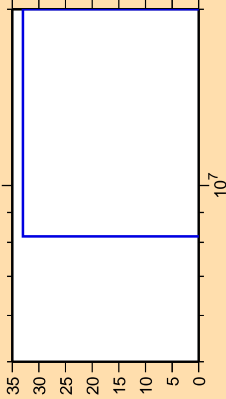
\Delta\sigma/\sigma vs. E for ^{185}\text{Ir}(n,p)
