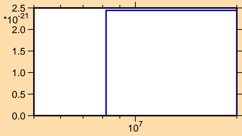
\sigma vs. E for ^{185}\text{Ir}(\text{mt } 42)
