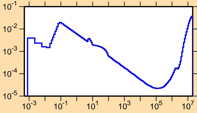
\sigma vs. E for ^{186}\text{Ir}(n,p)
