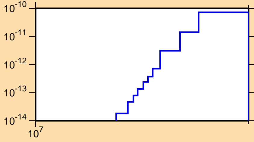
\sigma vs. E for ^{186}\text{Ir}(\text{mt117})
