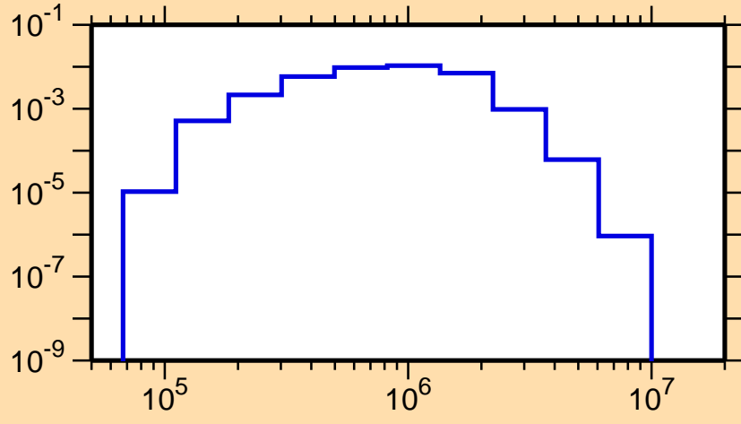
\sigma vs. E for ^{186}\text{Ir}(n,n_1)
