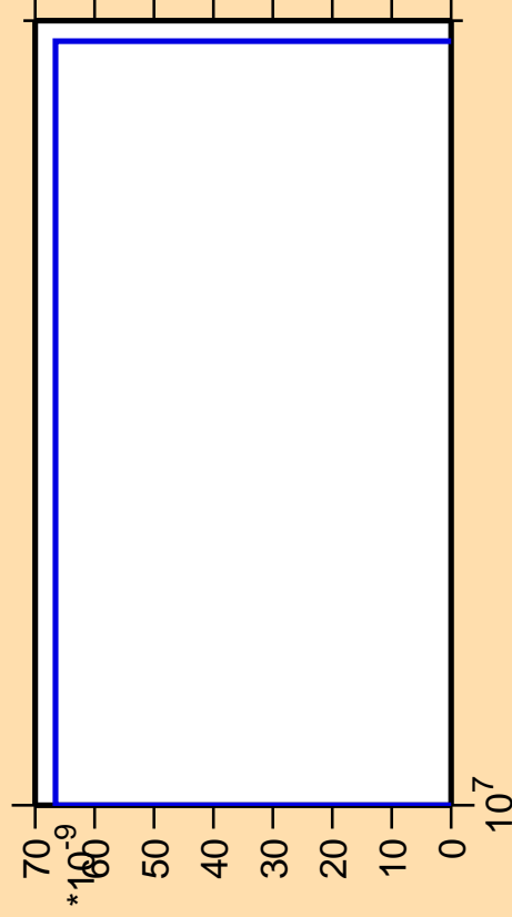
\Delta\sigma/\sigma vs. E for ^{186}\text{Ir} (mt 42)
