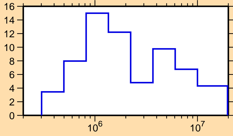
\Delta\sigma/\sigma vs. E for ^{186}\text{Ir}(n, el.)
