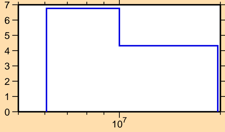
\Delta\sigma/\sigma vs. E for ^{186}\text{Ir}(n,\text{el.})
