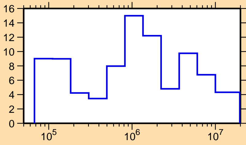
\Delta\sigma/\sigma vs. E for ^{186}\text{Ir}(n,\text{el.})
