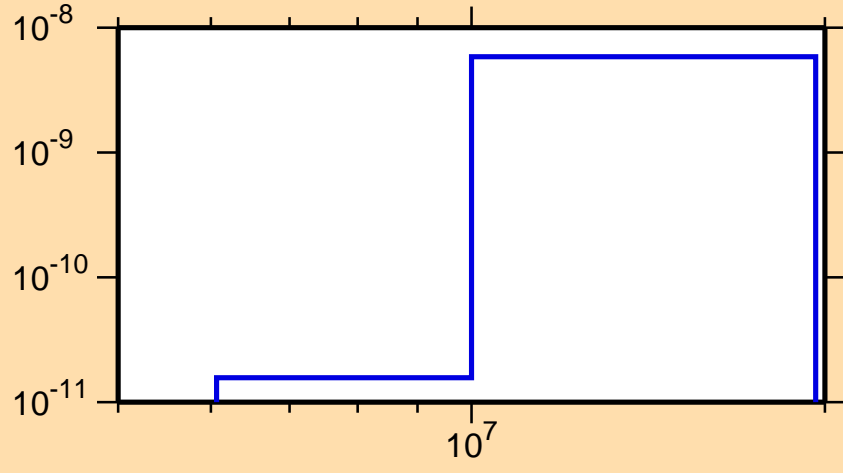
\sigma vs. E for ^{186}\text{Ir}(n,p\alpha)
