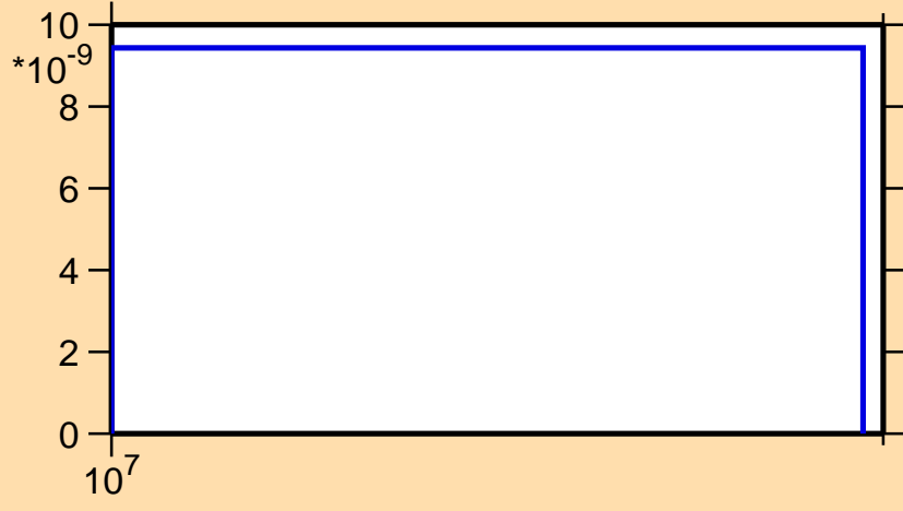
\sigma vs. E for ^{186}\text{Ir}(n,nt)
