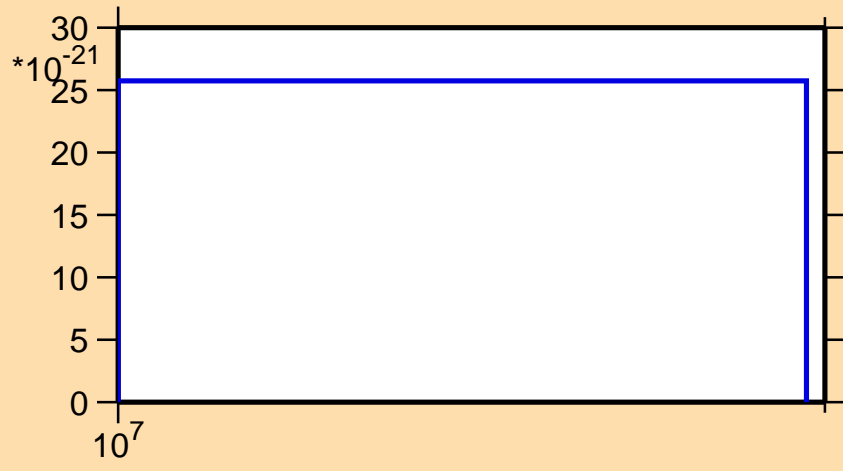
\sigma vs. E for ^{186}\text{Ir} (mt 42)
