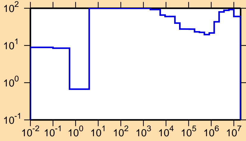
\Delta\sigma/\sigma vs. E for ^{186}\text{Ir}(n,\gamma)
