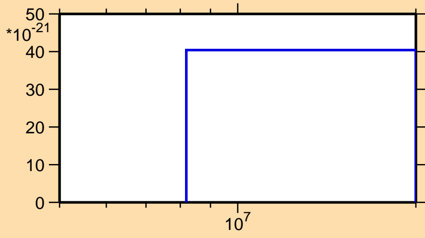
\sigma vs. E for ^{186}\text{Ir}(\text{mt } 42)
