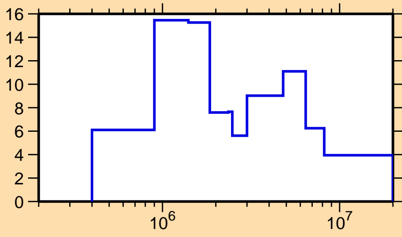
\Delta\sigma/\sigma vs. E for ^{186}\text{Ir}(n, el.)
