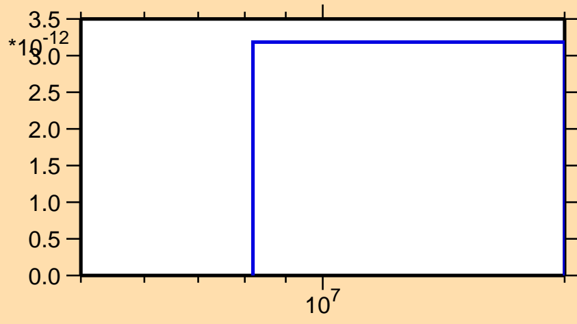
\sigma vs. E for ^{186}\text{Ir}(\text{mt } 45)
