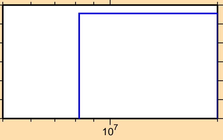
\sigma vs. E for ^{186}\text{Ir}(n,\text{He3})
