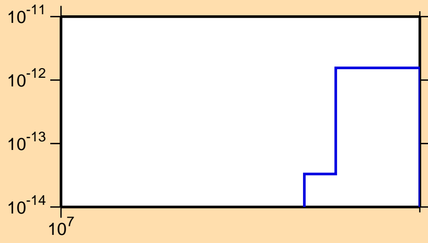
\sigma vs. E for ^{186}\text{Ir}(n,\text{pd})
