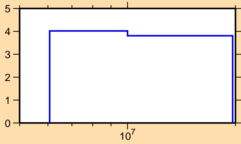
\Delta\sigma/\sigma vs. E for ^{186}\text{Ir}(n,\text{nonel.})
