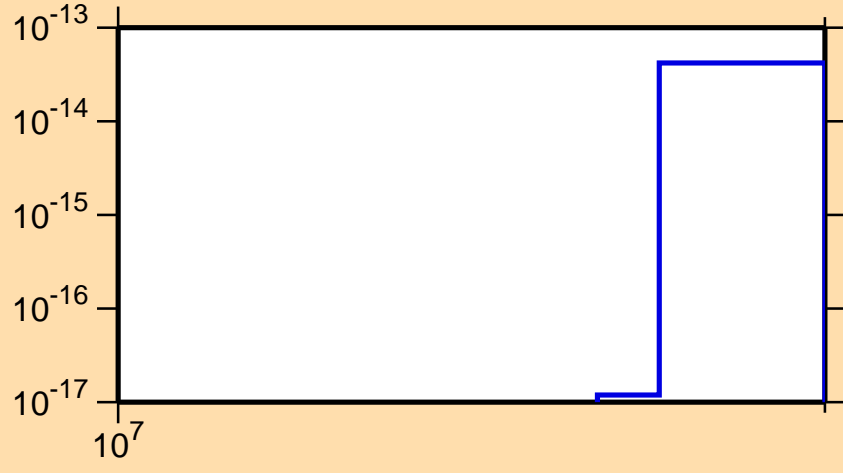
\sigma vs. E for ^{187}\text{Ir} (mt 34)
