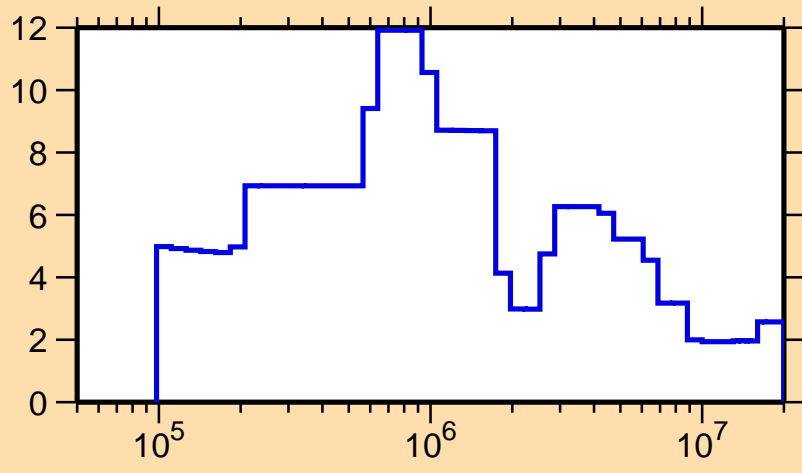
\Delta\sigma/\sigma vs. E for ^{187}\text{Ir}(n,\text{tot.})
