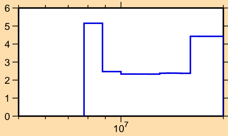
\Delta\sigma/\sigma vs. E for ^{187}\text{Ir}(n,\text{el.})
