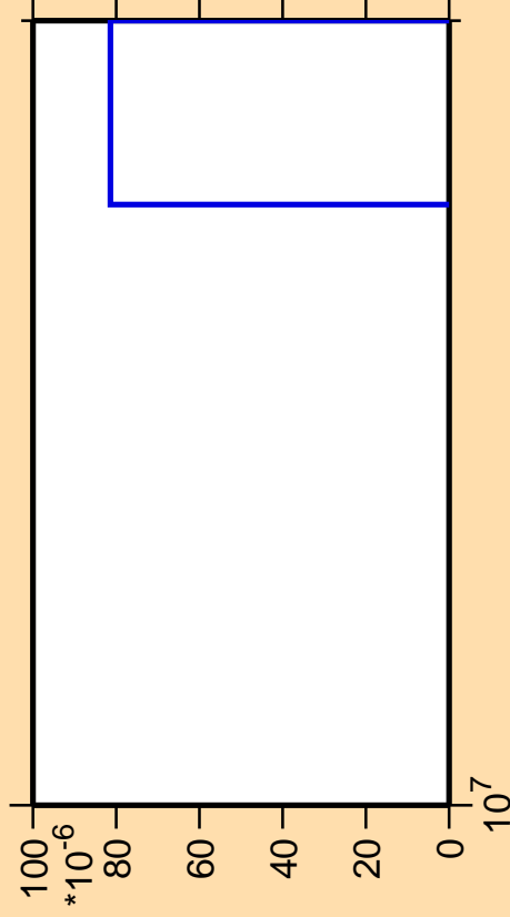
\Delta\sigma/\sigma vs. E for ^{187}\text{Ir} (mt 42)
