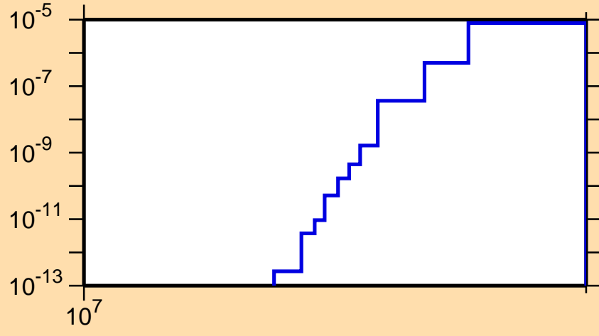
\sigma vs. E for ^{187}\text{Ir}(n,\text{nd})
