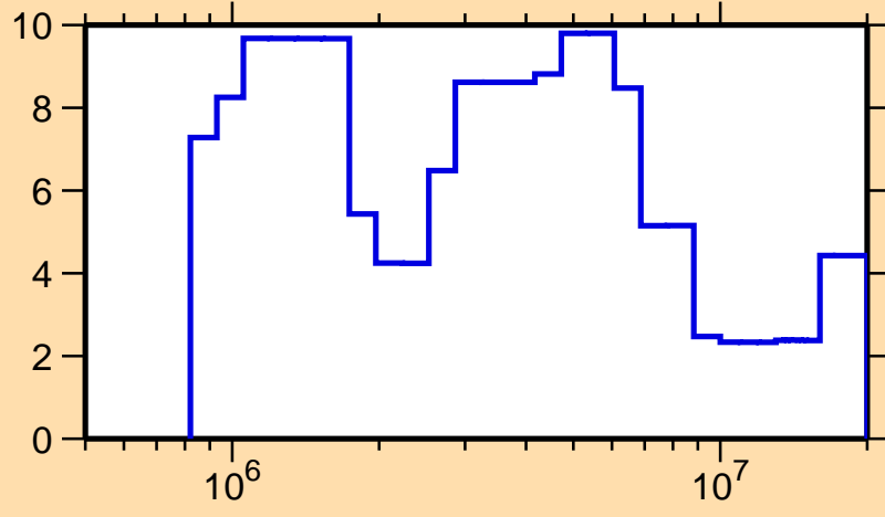
\Delta\sigma/\sigma vs. E for ^{187}\text{Ir}(n,el.)
