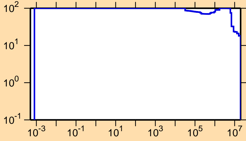
\Delta\sigma/\sigma vs. E for ^{187}\text{Ir}(n,p)
