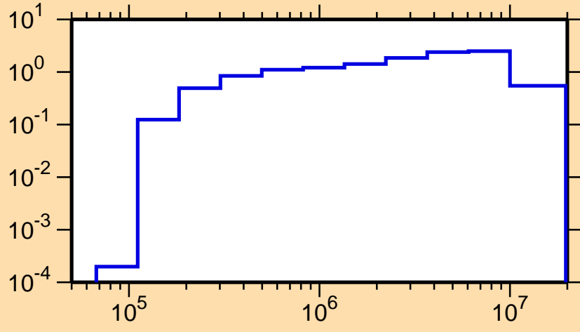
\sigma vs. E for ^{187}\text{Ir}(n,\text{inel.})
