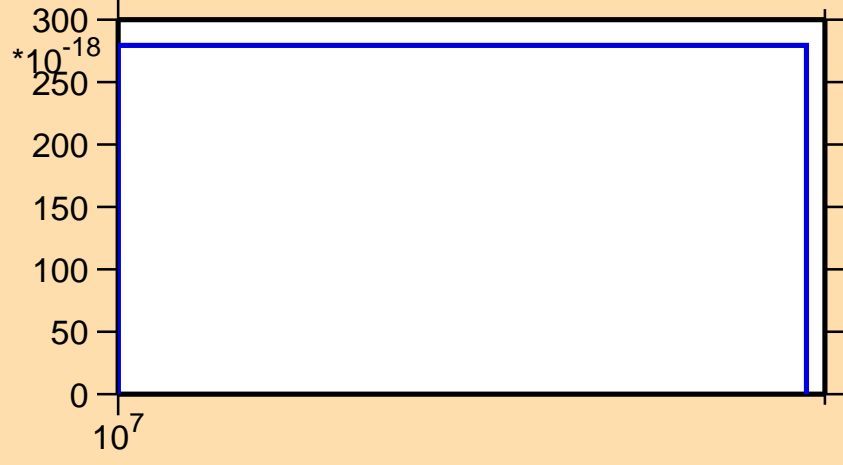
\sigma vs. E for ^{187}\text{Ir} (mt 34)
