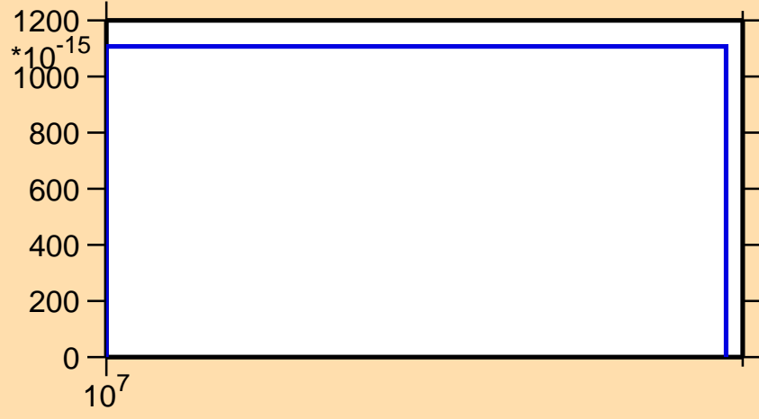
\sigma vs. E for ^{187}\text{Ir} (mt 45)
