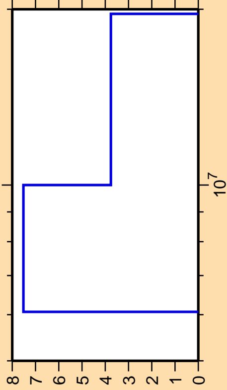
\Delta\sigma/\sigma vs. E for ^{187}\text{Ir}(n,2n)
