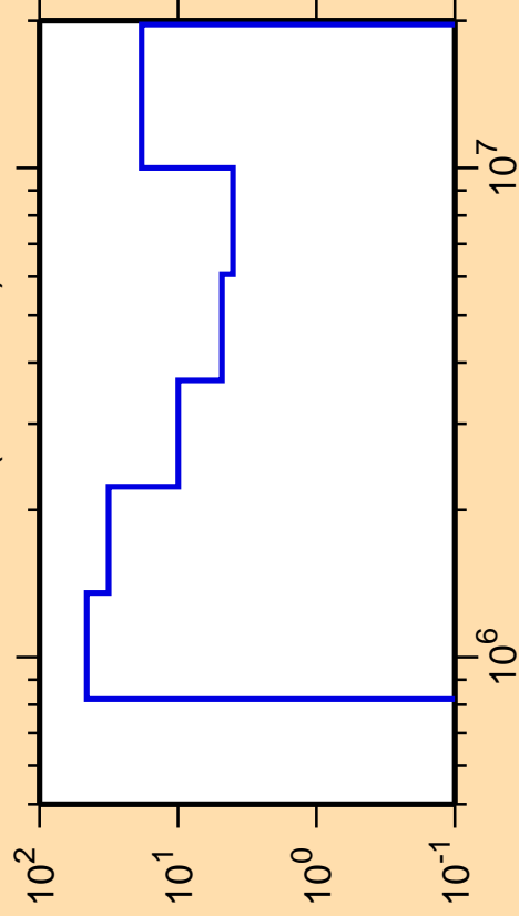
\Delta\sigma/\sigma vs. E for ^{187}\text{Ir}(n,n\text{cont.})
