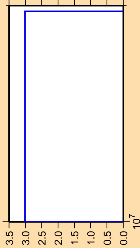
\Delta\sigma/\sigma vs. E for ^{187}\text{Ir} (mt 45)
