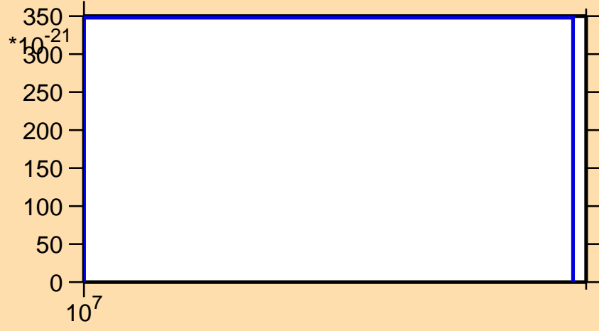
\sigma vs. E for ^{187}\text{Ir} (mt 42)
