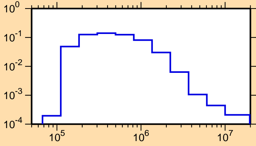
\sigma vs. E for ^{187}\text{Ir}(n,n_1)
