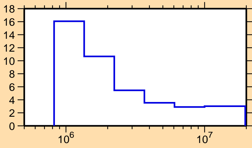
\Delta\sigma/\sigma vs. E for ^{187}\text{Ir}(n,n\text{onel.})
