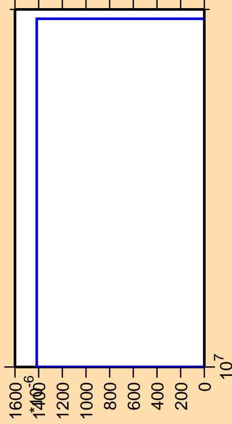
\Delta\sigma/\sigma vs. E for ^{187}\text{Ir} (mt 34)
