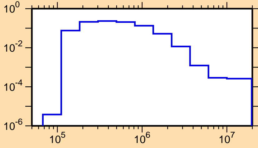
\sigma vs. E for ^{187}\text{Ir}(n,n_2)
