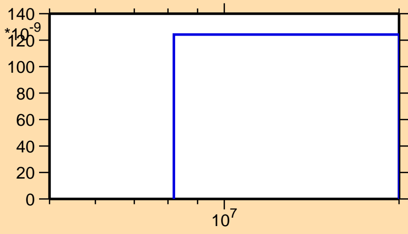
\sigma vs. E for ^{187}\text{Ir}(n,2np)
