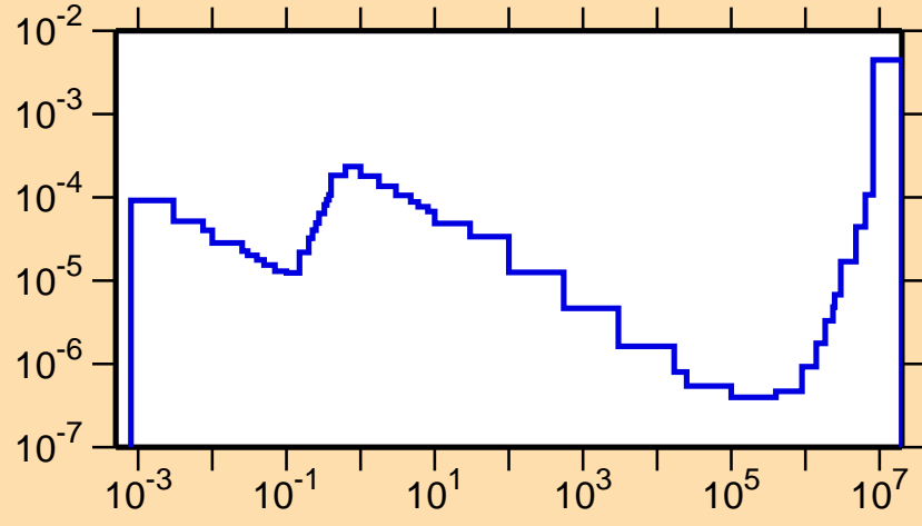
\sigma vs. E for ^{187}\text{Ir}(n,\alpha)
