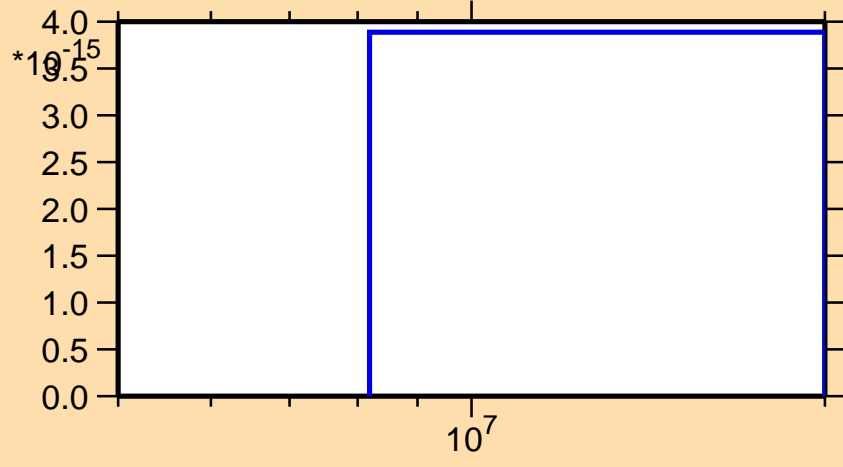
\sigma vs. E for ^{188}\text{Ir}(\text{mt } 34)
