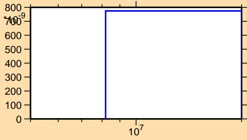
\sigma vs. E for ^{188}\text{Ir}(n,2n\alpha)
