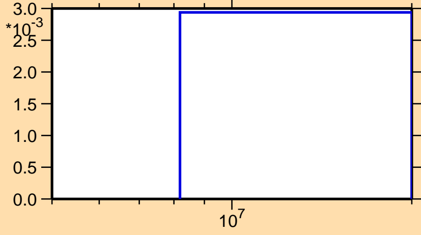
\sigma vs. E for ^{188}\text{Ir}(n,3n)
