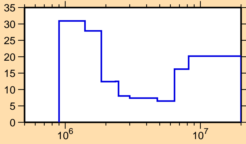
\Delta\sigma/\sigma vs. E for ^{188}\text{Ir}(n,ncont.)
