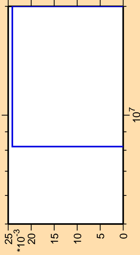
\Delta\sigma/\sigma vs. E for ^{188}\text{Ir}(\text{mt } 34)
