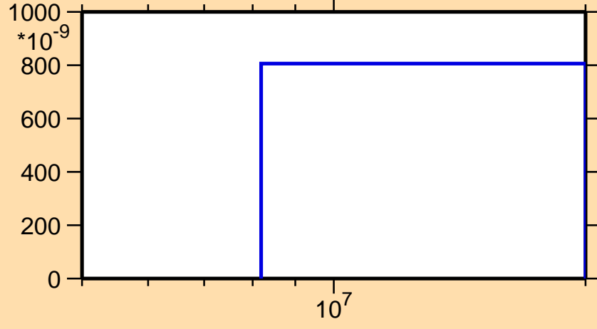
\sigma vs. E for ^{188}\text{Ir}(n,\text{nd})
