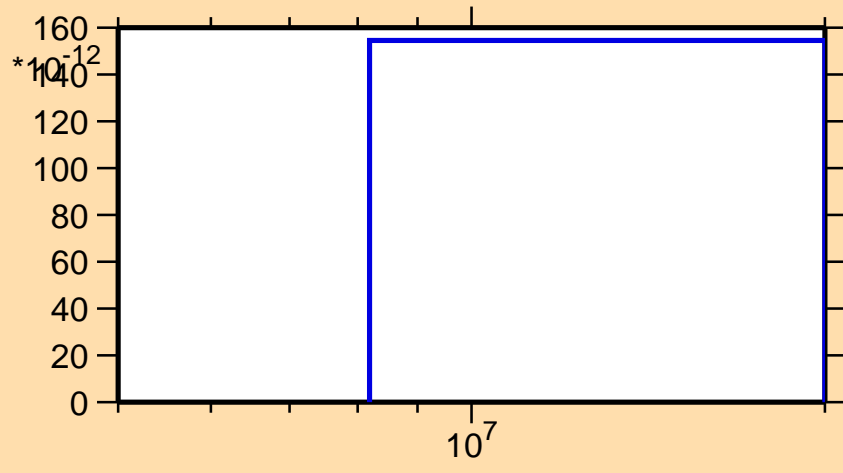
\sigma vs. E for ^{188}\text{Ir}(n,p\alpha)
