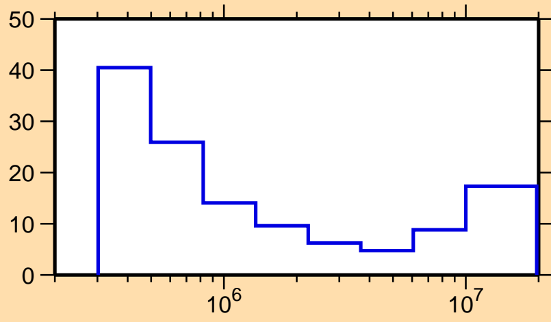
\Delta\sigma/\sigma vs. E for ^{190}\text{Ir}(n,n\text{cont.})
