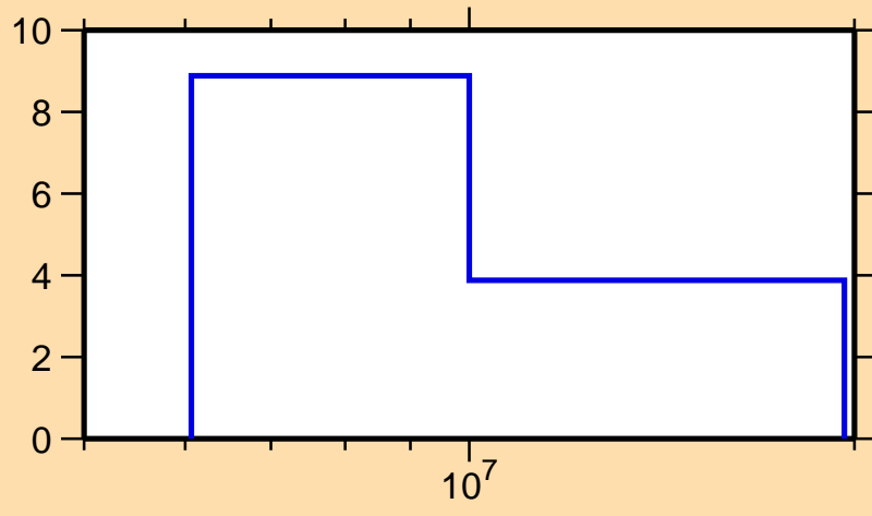
\Delta\sigma/\sigma vs. E for ^{190}\text{Ir}(n,2n)
