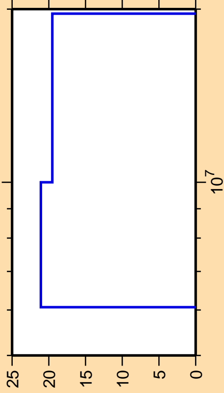
\Delta\sigma/\sigma vs. E for ^{190}\text{Ir}(n,p)
