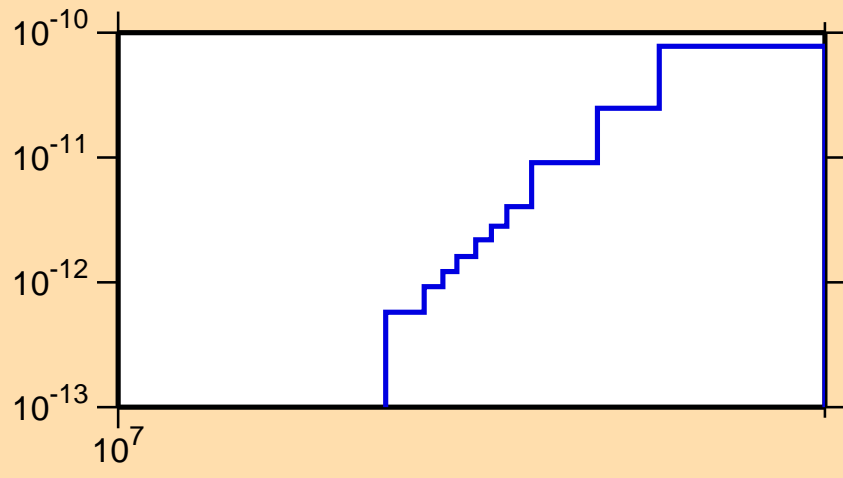
\sigma vs. E for ^{190}\text{Ir}(n,p\alpha)
