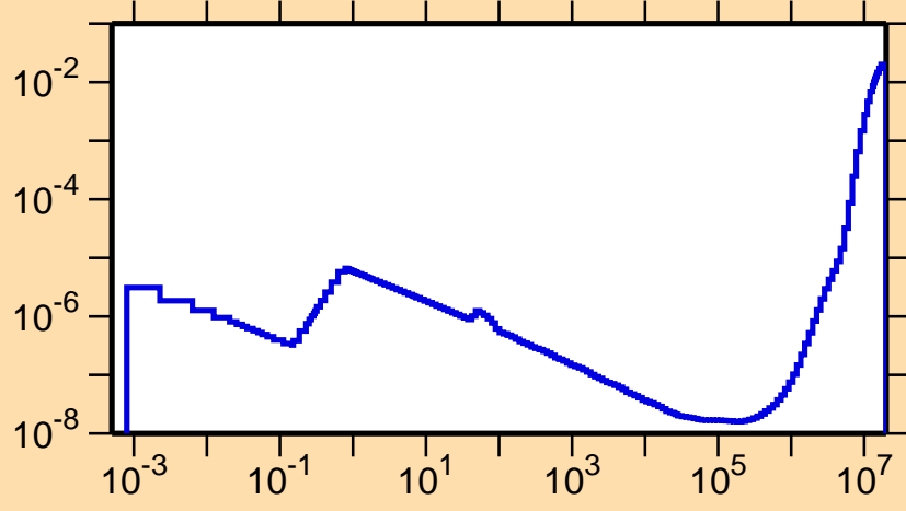
\sigma vs. E for ^{190}\text{Ir}(n,p)
