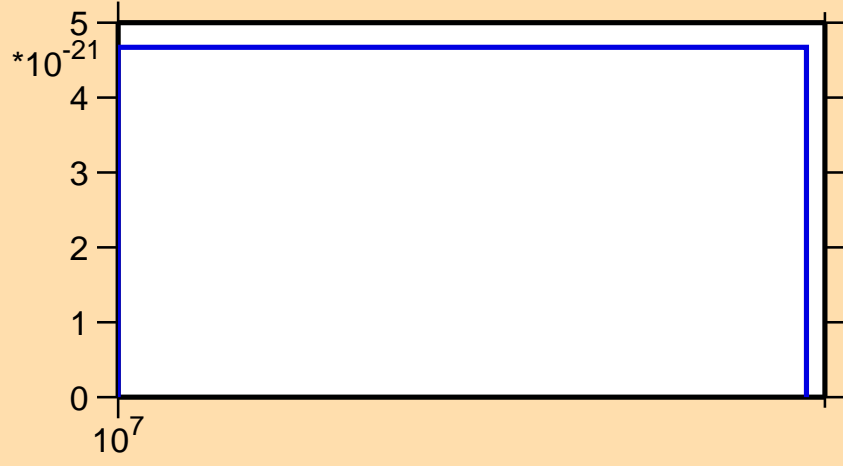
\sigma vs. E for ^{190}\text{Ir} (mt 42)
