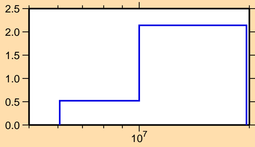
\sigma vs. E for ^{190}\text{Ir}(n,2n)
