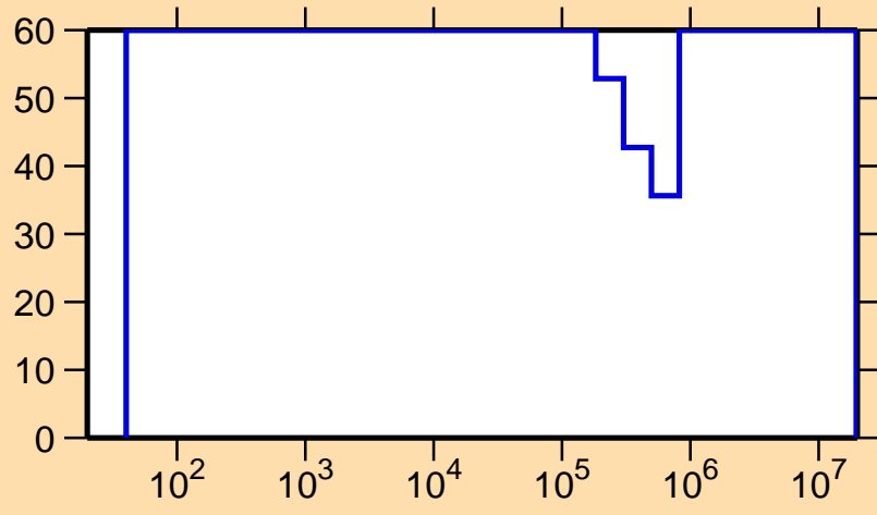
\Delta\sigma/\sigma vs. E for ^{190}\text{Ir}(n,n_1)
