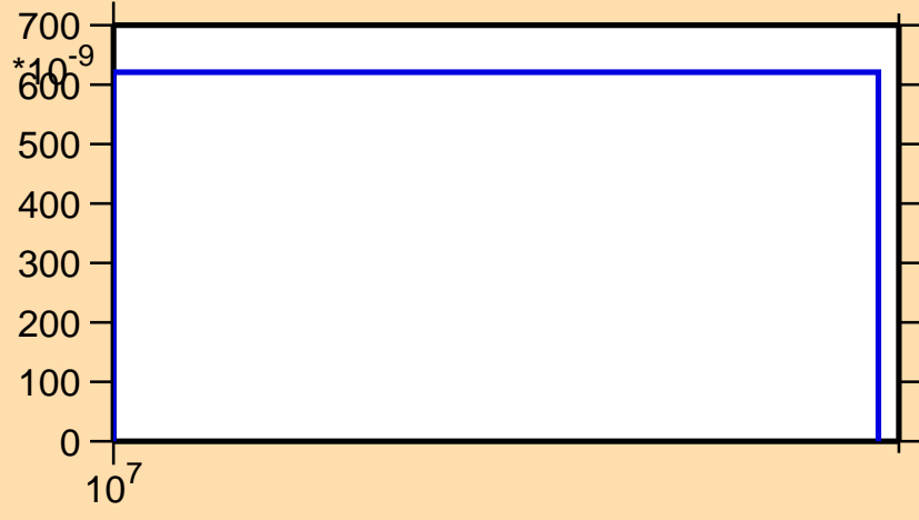
\sigma vs. E for ^{190}\text{Ir}(n,\text{nd})
