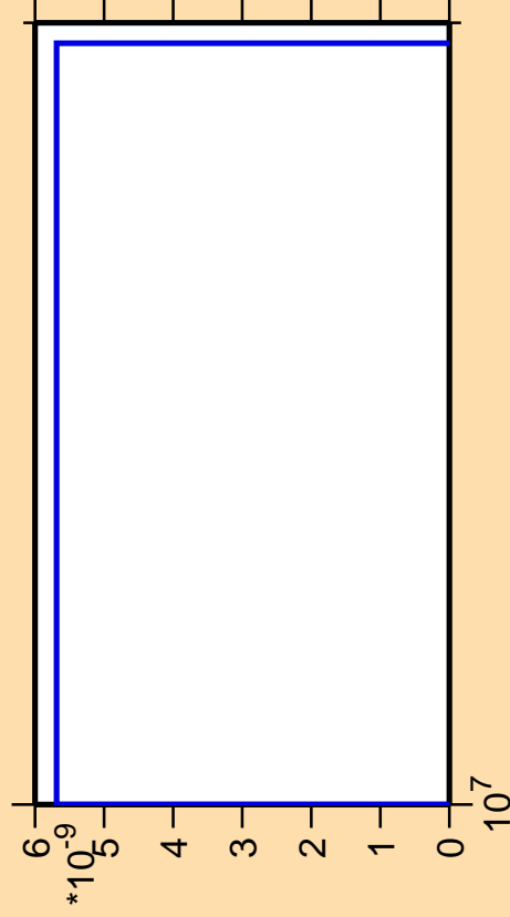
\Delta\sigma/\sigma vs. E for ^{190}\text{Ir} (mt 42)
