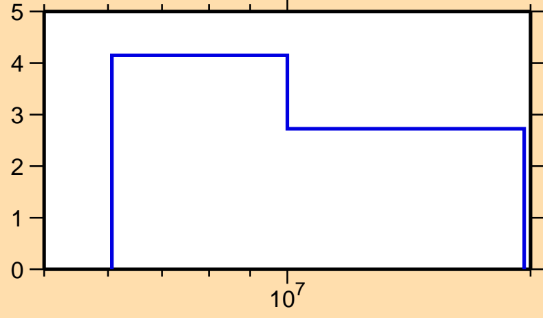
\Delta\sigma/\sigma vs. E for ^{190}\text{Ir}(n,\text{el.})
