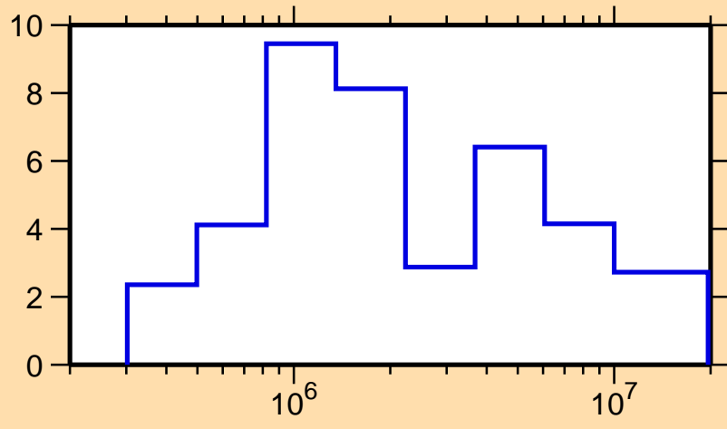
\Delta\sigma/\sigma vs. E for ^{190}\text{Ir}(n, el.)
