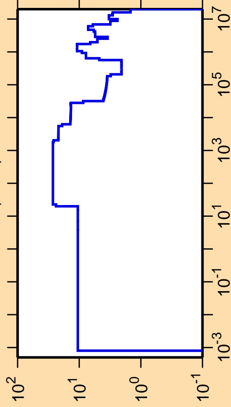
\Delta\sigma/\sigma vs. E for ^{190}\text{Ir}(n,\text{el.})
