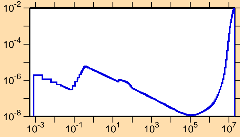
\sigma vs. E for ^{190}\text{Ir}(n,\alpha)
