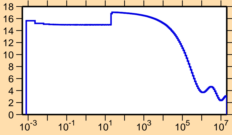
\sigma vs. E for ^{190}\text{Ir}(n,\text{el.})
