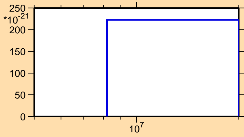
\sigma vs. E for ^{190}\text{Ir}(\text{mt } 42)
