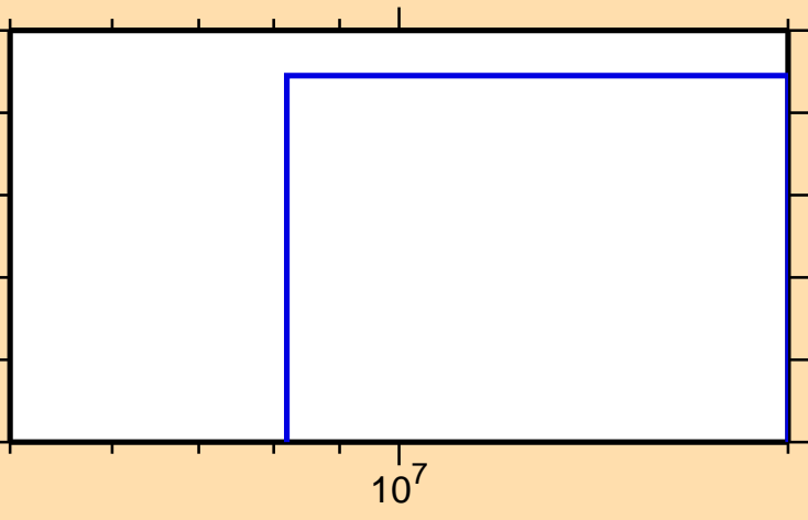
\sigma vs. E for ^{190}\text{Ir}(\text{mt } 42)
