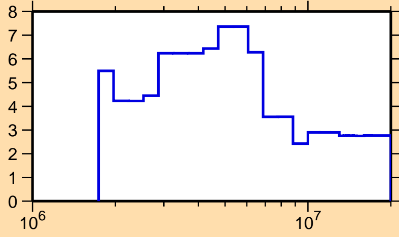
\Delta\sigma/\sigma vs. E for ^{191}\text{Ir}(n,el.)
