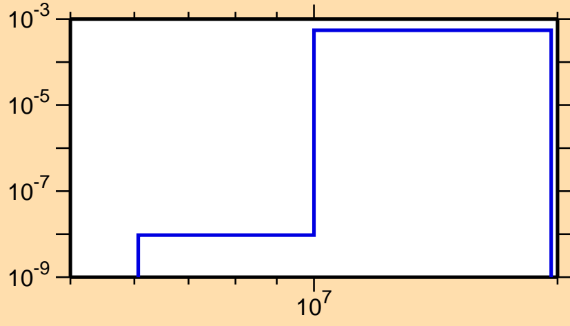
\sigma vs. E for ^{191}\text{Ir}(n,np)
