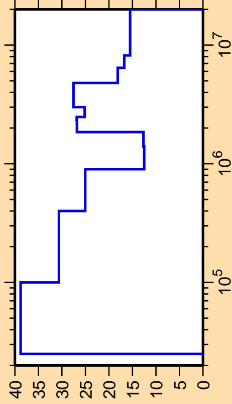
\Delta\sigma/\sigma vs. E for ^{191}\text{Ir}(n,n_1)
