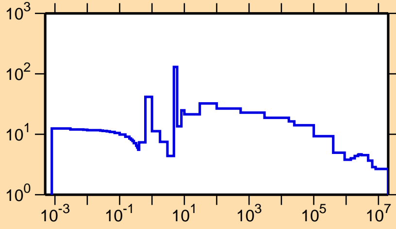
\sigma vs. E for ^{191}\text{Ir}(n,\text{el.})
