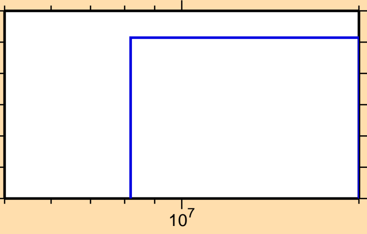
\sigma vs. E for ^{191}\text{Ir}(\text{mt } 42)
