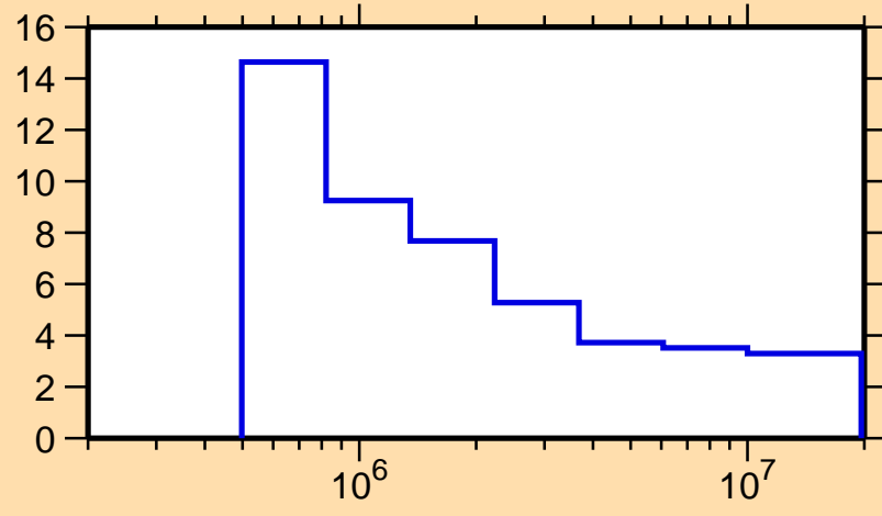
\Delta\sigma/\sigma vs. E for ^{191}\text{Ir}(n,n\text{onel.})
