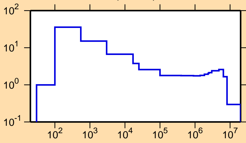
\sigma vs. E for ^{191}\text{Ir}(n,\text{inel.})
