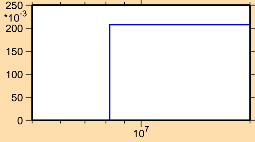
\sigma vs. E for ^{191}\text{Ir}(n,3n)
