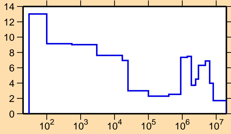
\Delta\sigma/\sigma vs. E for ^{191}\text{Ir}(n, el.)
