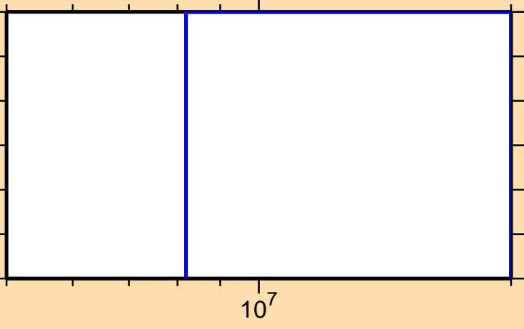
\sigma vs. E for ^{192}\text{Ir}(n,nt)
