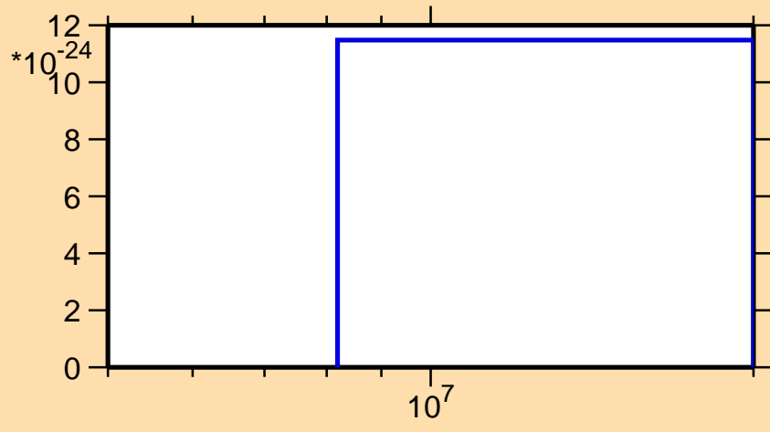
\sigma vs. E for ^{192}\text{Ir}(\text{mt } 42)
