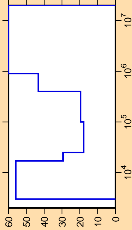
\Delta\sigma/\sigma vs. E for ^{192}\text{Ir}(n,n_2)
