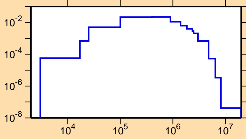
\sigma vs. E for ^{192}\text{Ir}(n,n_4)
