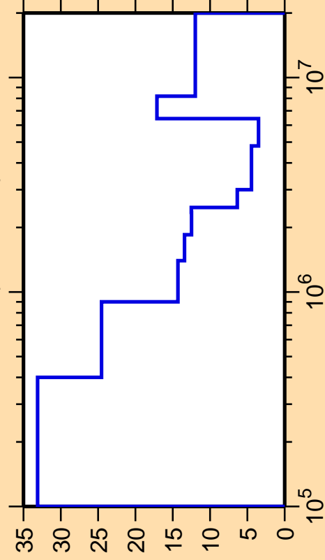
\Delta\sigma/\sigma vs. E for ^{192}\text{Ir}(n,n\text{cont.})
