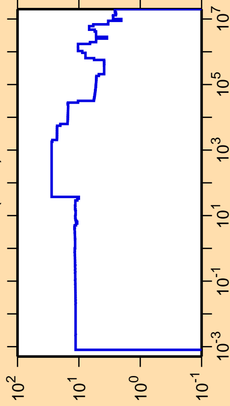
\Delta\sigma/\sigma vs. E for ^{192}\text{Ir}(n,\text{el.})
