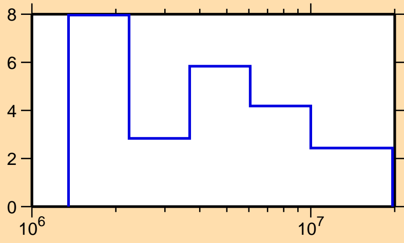
\Delta\sigma/\sigma vs. E for ^{192}\text{Ir}(n,\text{el.})
