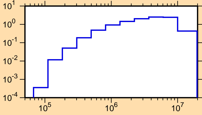
\sigma vs. E for ^{192}\text{Ir}(n,n\text{cont.})
