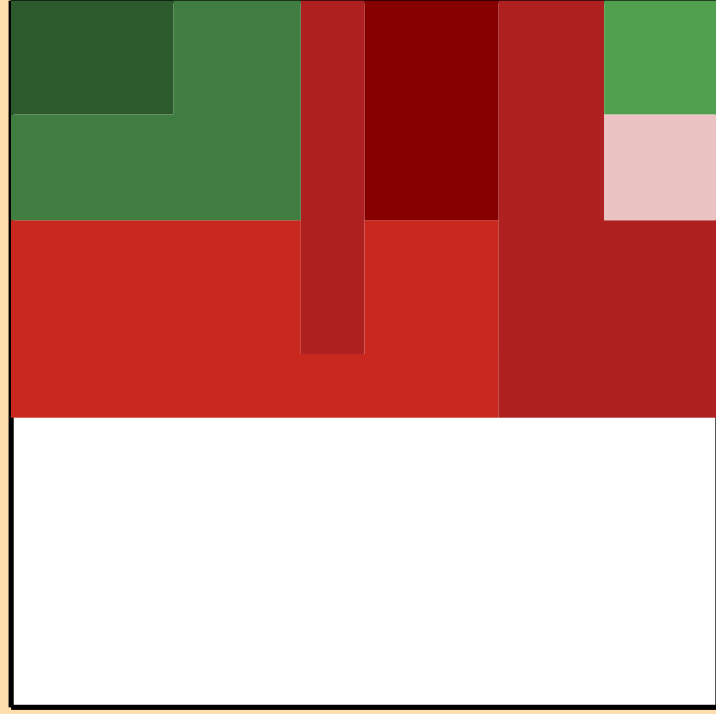
\Delta\sigma/\sigma vs. E for ^{193}\text{Ir}(n,\text{el.})
