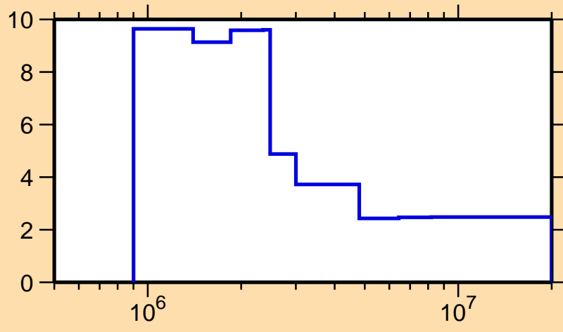
\Delta\sigma/\sigma vs. E for ^{193}\text{Ir}(n, n_{\text{nonel}})
