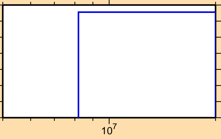
\sigma vs. E for ^{193}\text{Ir}(n,nt)
