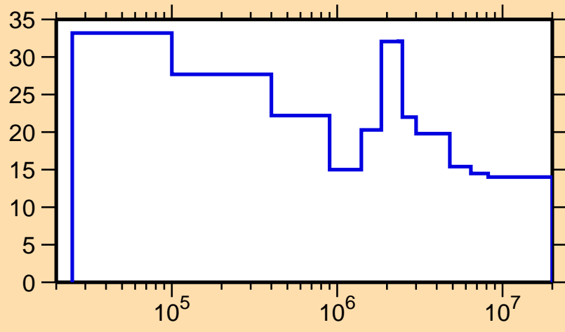
\Delta\sigma/\sigma vs. E for ^{193}\text{Ir}(n,n_1)
