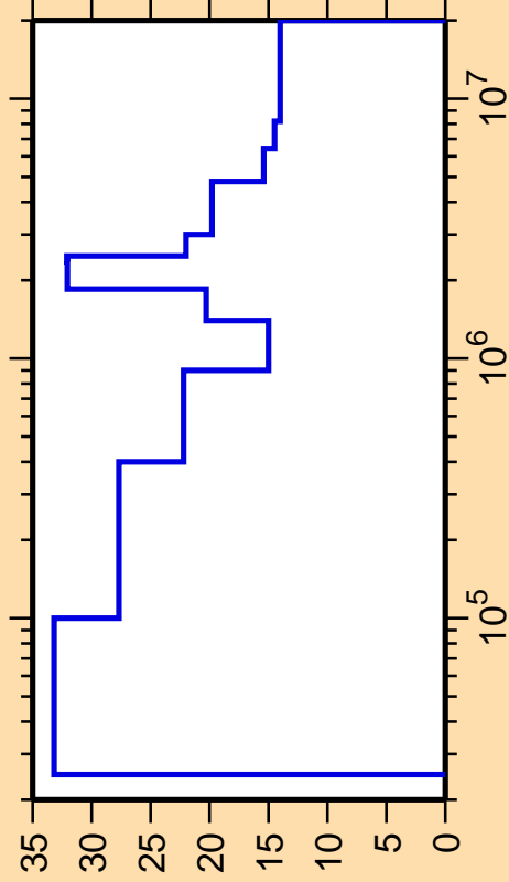
\Delta\sigma/\sigma vs. E for ^{193}\text{Ir}(n,n_1)
