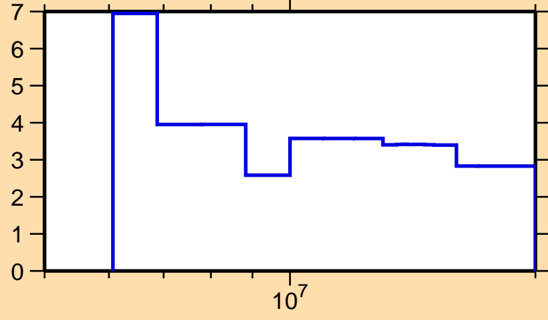
\Delta\sigma/\sigma vs. E for ^{194}\text{Ir}(n,\text{el.})
