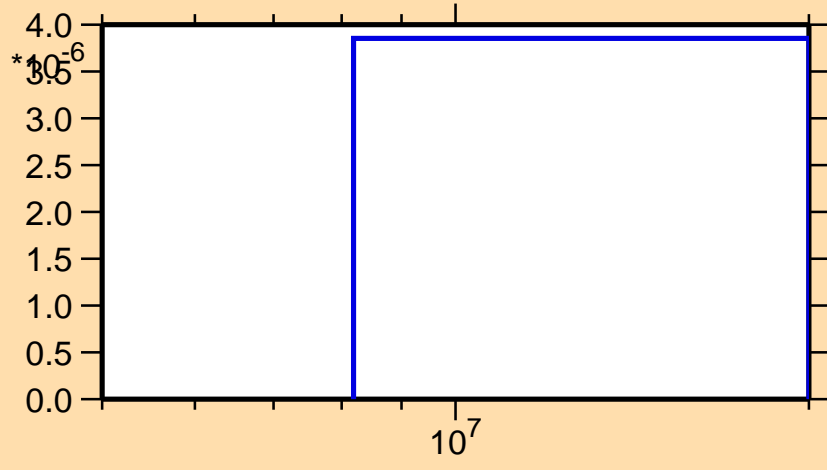
\sigma vs. E for ^{194}\text{Ir}(n,n\alpha)
