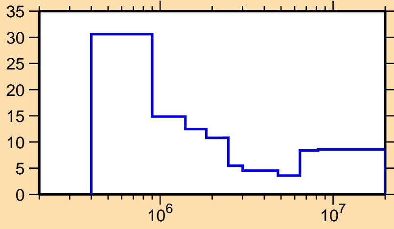
\Delta\sigma/\sigma vs. E for ^{194}\text{Ir}(n,n\text{cont.})
