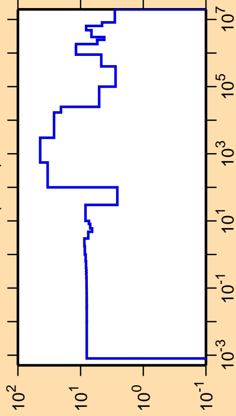
\Delta\sigma/\sigma vs. E for ^{194}\text{Ir}(n,\text{el.})
