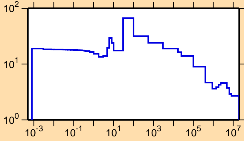
\sigma vs. E for ^{194}\text{Ir}(n,\text{el.})
