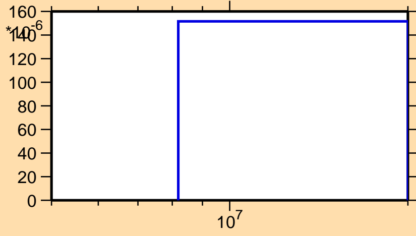
\sigma vs. E for ^{194}\text{Ir}(n,np)
