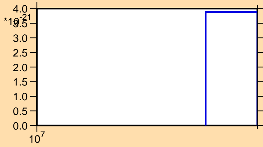
\sigma vs. E for ^{194}\text{Ir} (mt 42)
