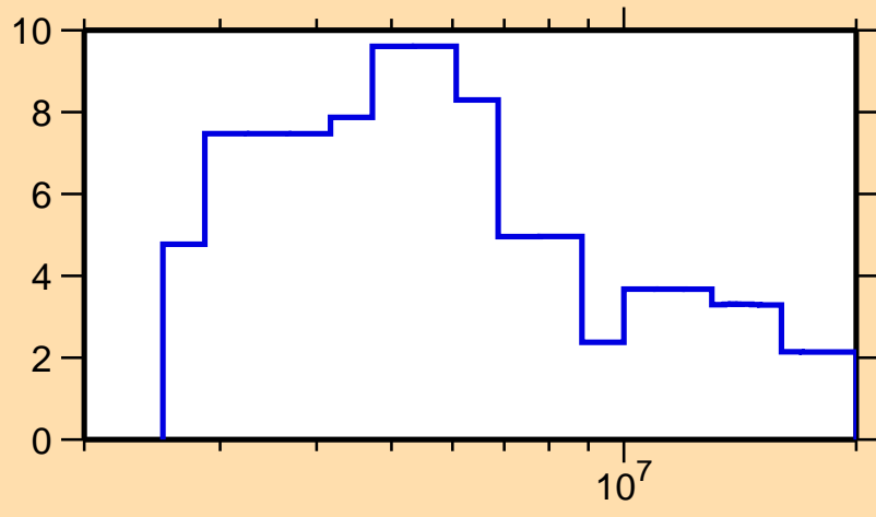
\Delta\sigma/\sigma vs. E for ^{194}\text{Ir}(n,el.)
