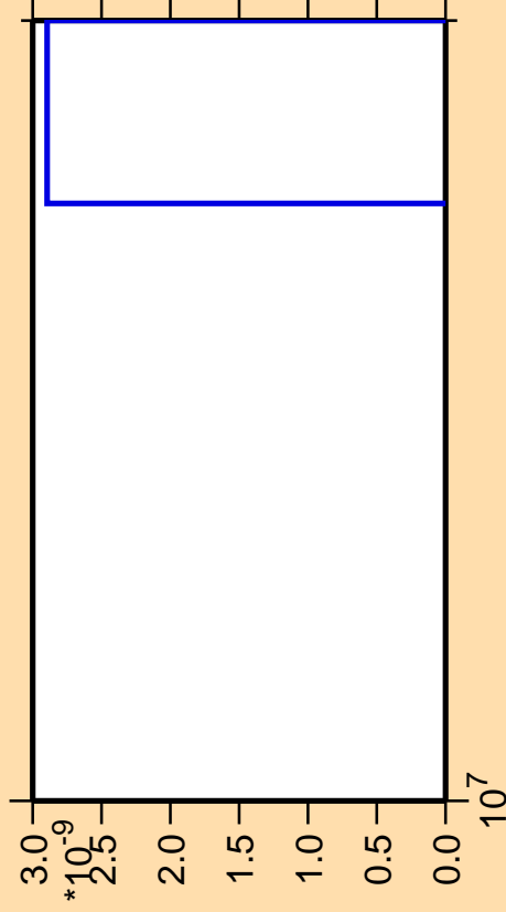
\Delta\sigma/\sigma vs. E for ^{194}\text{Ir} (mt 42)
