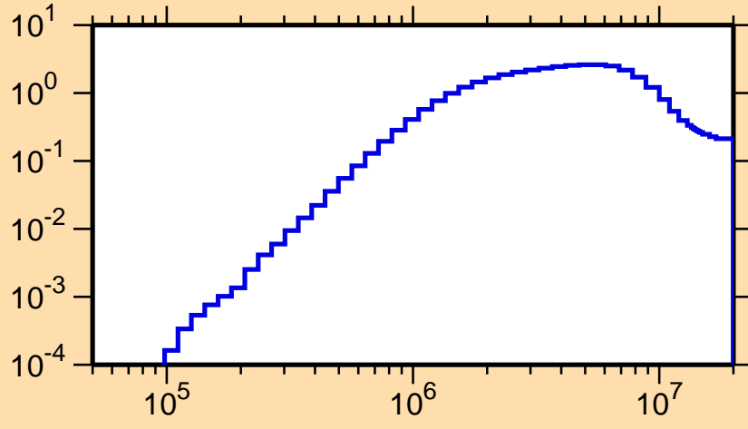
\sigma vs. E for ^{194}\text{Ir}(n,n\text{cont.})
