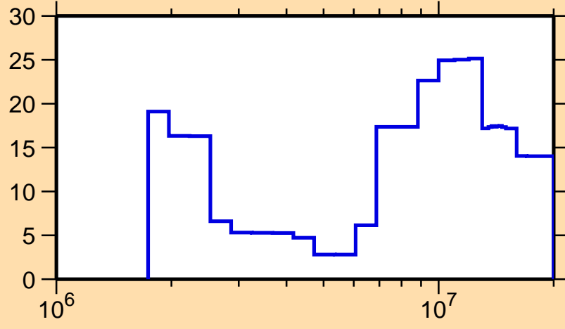
\Delta\sigma/\sigma vs. E for ^{194}\text{Ir}(n,n\text{cont.})
