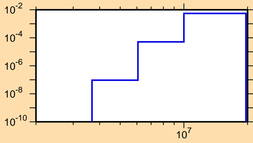
\sigma vs. E for ^{194}\text{Ir}(n,p)
