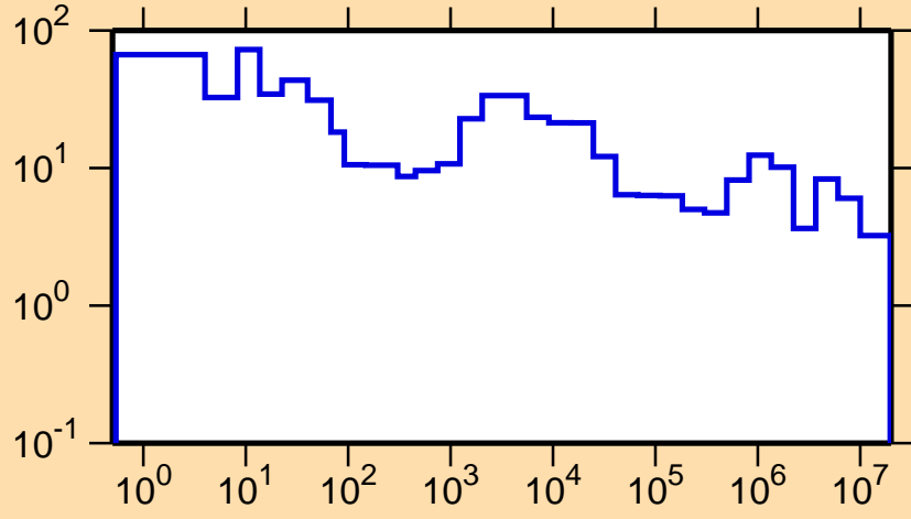
\Delta\sigma/\sigma vs. E for ^{194}\text{Ir}(n, el.)
