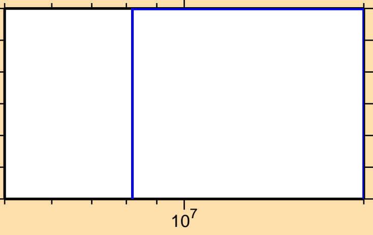
\sigma vs. E for ^{194}\text{Ir}(n,\text{nd})
