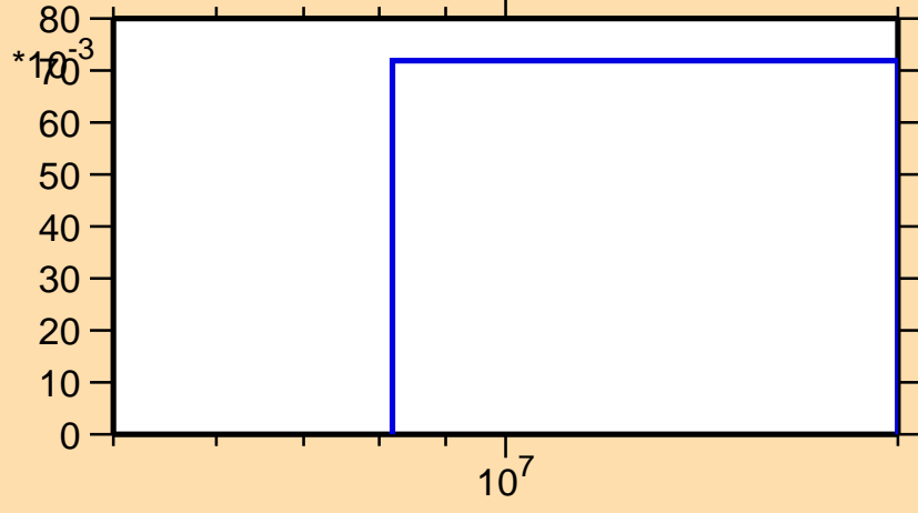
\sigma vs. E for ^{194}\text{Ir}(n,3n)
