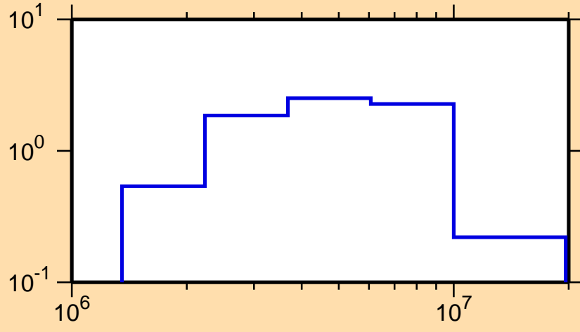
\sigma vs. E for ^{195}\text{Ir}(n,n\text{cont.})
