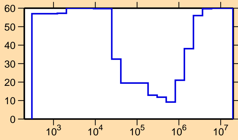
\Delta\sigma/\sigma vs. E for ^{195}\text{Ir}(n,n_1)
