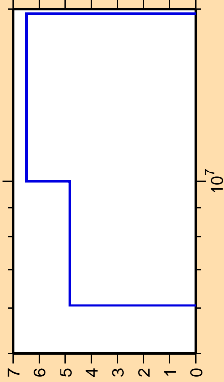
\Delta\sigma/\sigma vs. E for ^{195}\text{Ir}(n,2n)
