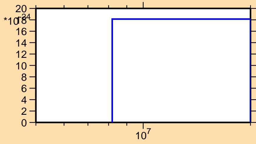
\sigma vs. E for ^{195}\text{Ir}(\text{mt } 42)
