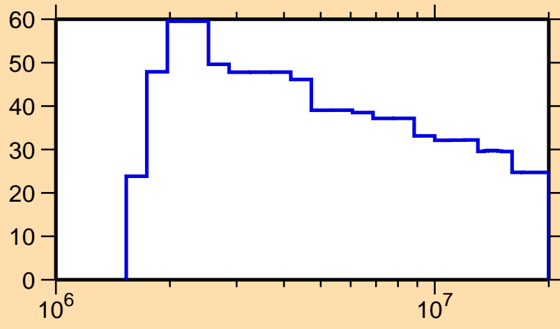
\Delta\sigma/\sigma vs. E for ^{197}\text{Ir}(n,n_1)
