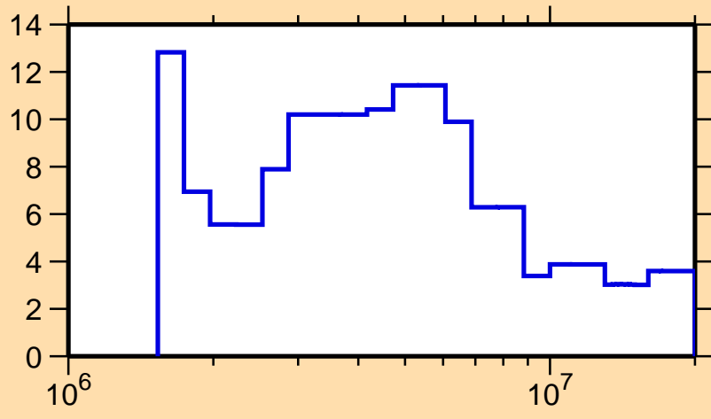
\Delta\sigma/\sigma vs. E for ^{197}\text{Ir}(n, el.)
