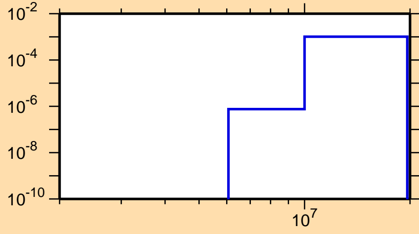
\sigma vs. E for ^{197}\text{Ir}(n,p)
