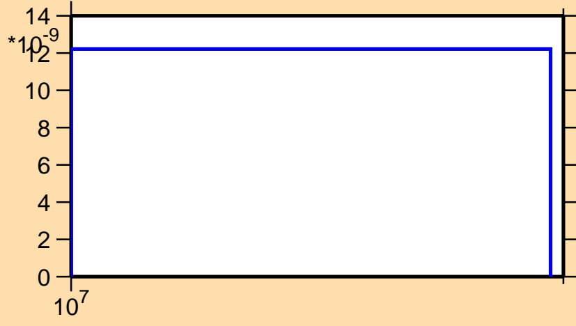
\sigma vs. E for ^{198}\text{Ir}(n,\text{nd})
