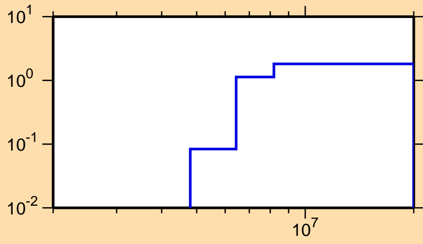
\sigma vs. E for ^{198}\text{Ir}(n,2n)
