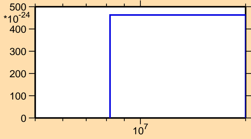
\sigma vs. E for ^{198}\text{Ir}(\text{mt } 42)
