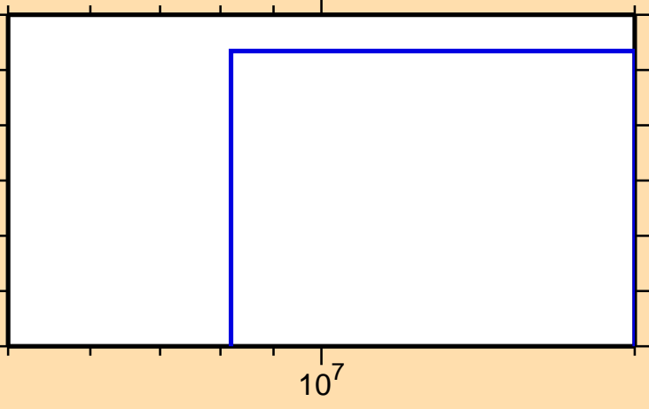
\sigma vs. E for ^{198}\text{Ir}(n,2np)
