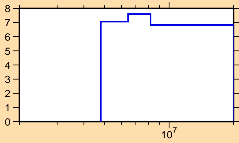
\Delta\sigma/\sigma vs. E for ^{198}\text{Ir}(n,\text{nonel.})
