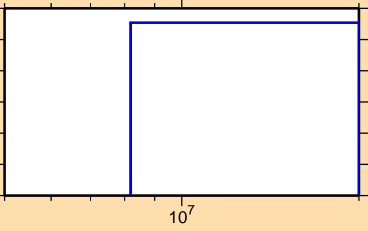
\sigma vs. E for ^{198}\text{Ir}(n,\text{nd})
