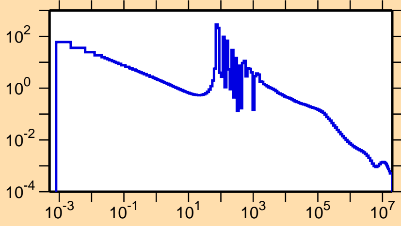
\sigma vs. E for ^{200}\text{Ir}(n,\gamma)
